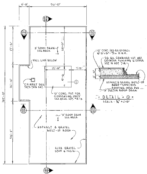
SECOND FLOOR ROOF PLAN SCALE: 1/8" = 1'-0"
