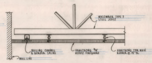
SUSPENDED - CEILING - DETAIL SCALE: 3/8" = 1'-0"
