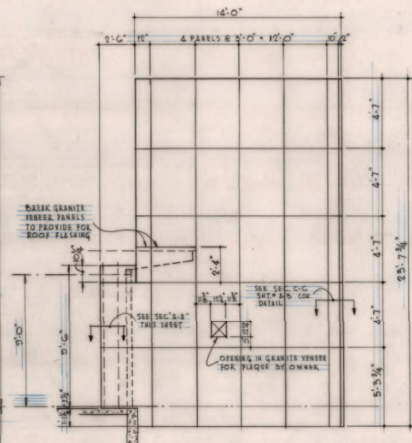
ELEV. GRANITE PANELS SOUTH WALL SCALE: 1/8" = 1'-0"
