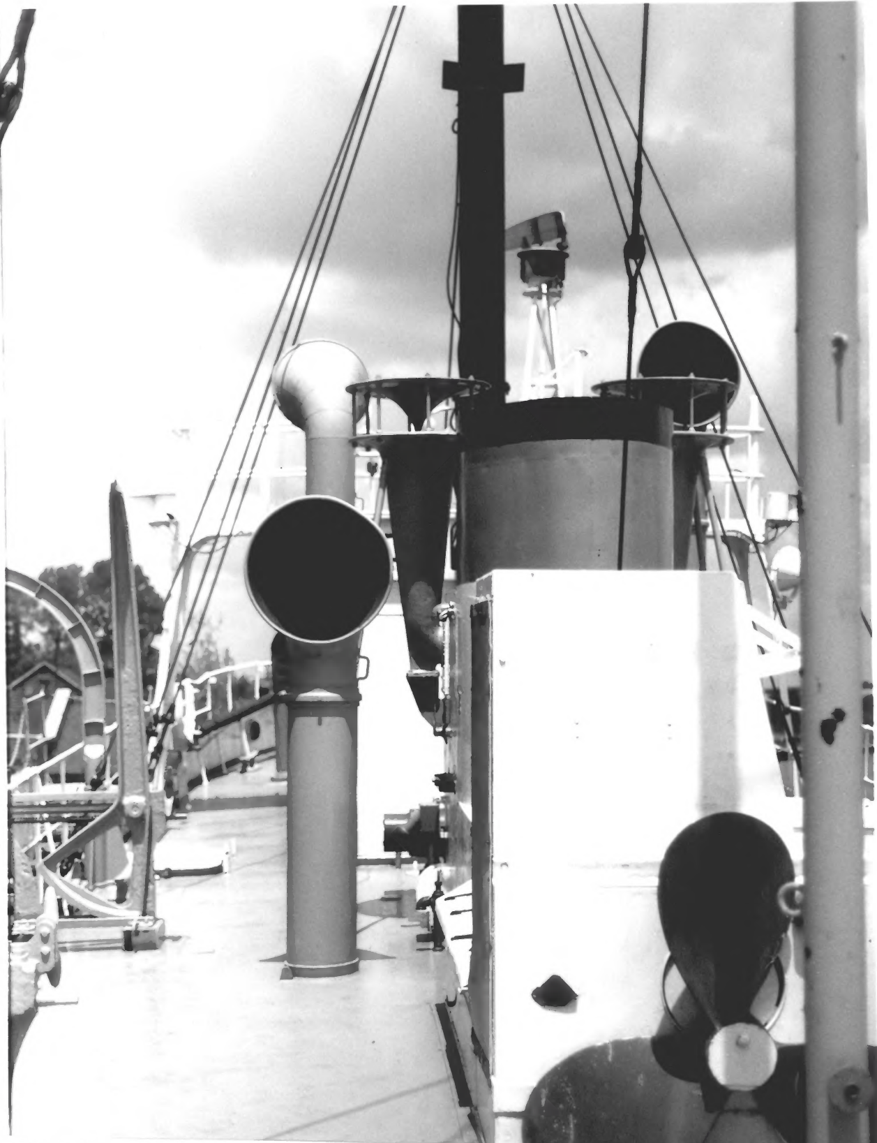
LIGHTSHIP NO. 103, HURON PORT HURON, MICHIGAN Owner: CITY OF PORT HURON DECK VIEW OF LIGHTSHIP NO. 103, LOOKING FORWARD. NOTE PROPELLER. Photo #4 by JAMES P. DELGADO, 1989 Courtesy of: NATIONAL PARK SERVICE
