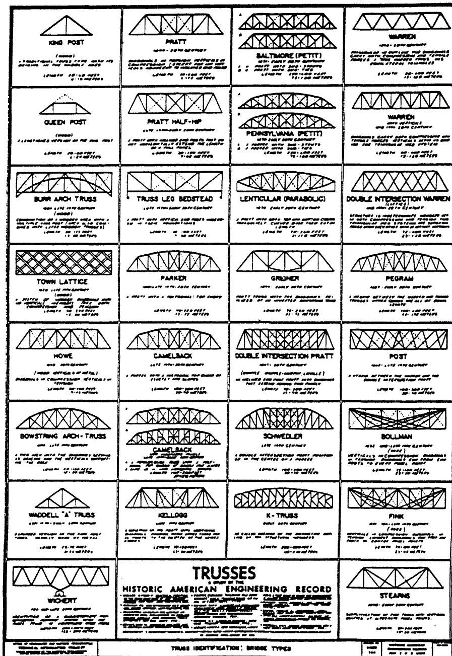
Historic American Engineering Record drawing showing the variety of 19 th and early-20 th century bridge designs. (1976)
