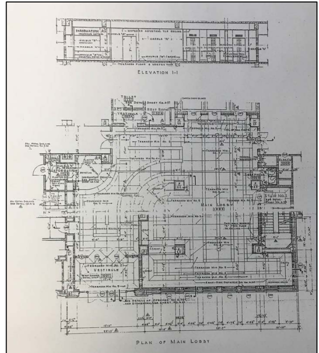
Figure 21. Detail of drawings for the lobby, Veterans Administration Hospital, in Wilmington, Delaware (VA).
