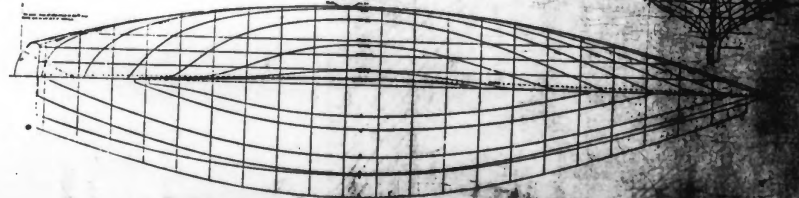
Auxiliary Schooner Adventuress. Designed by B. B. Crowninshield
