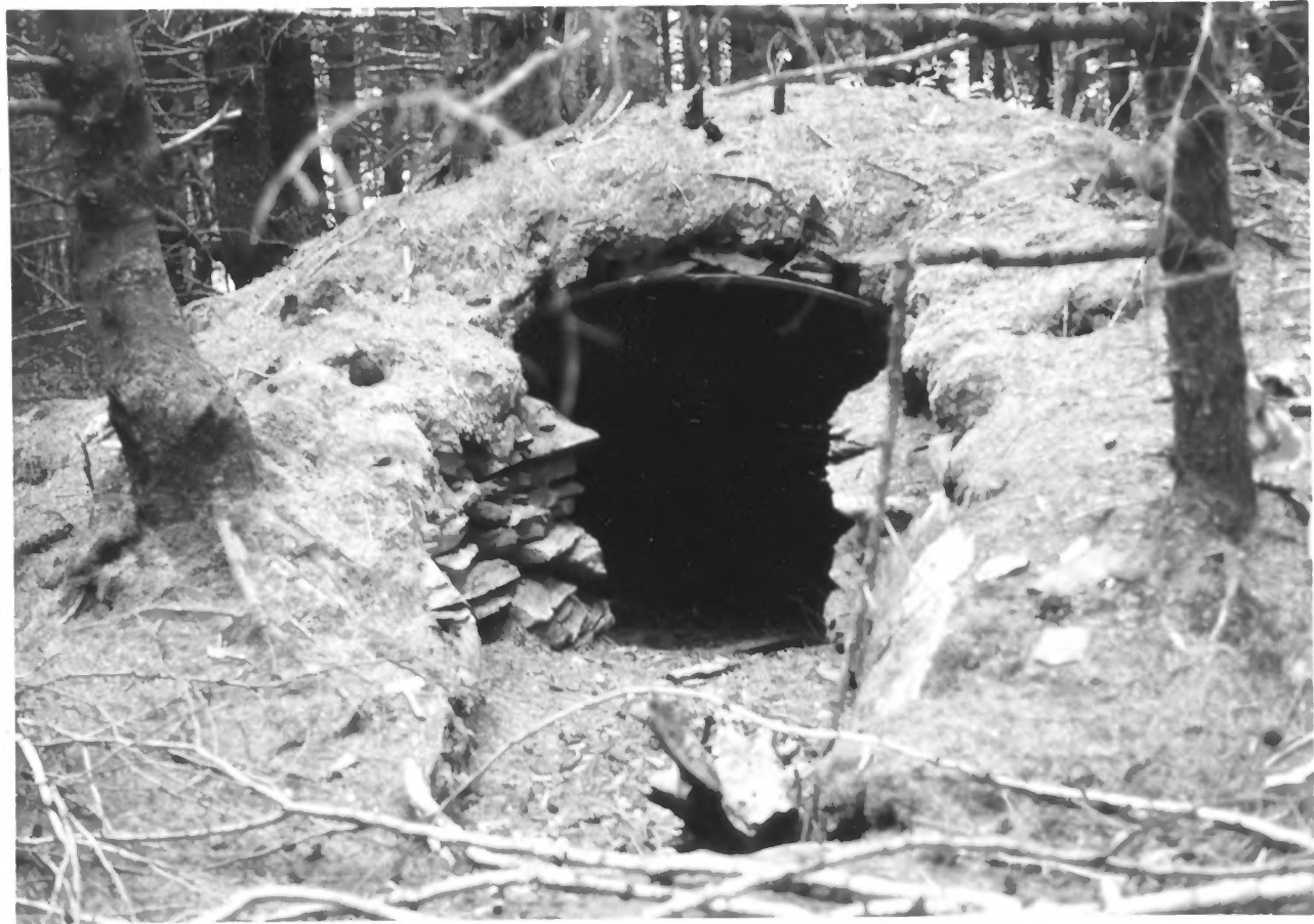
7. Personnel shelter, corrugated steel, rock, and earth. One of several in the vicinity of Artillery Hill, Fort Greely.
