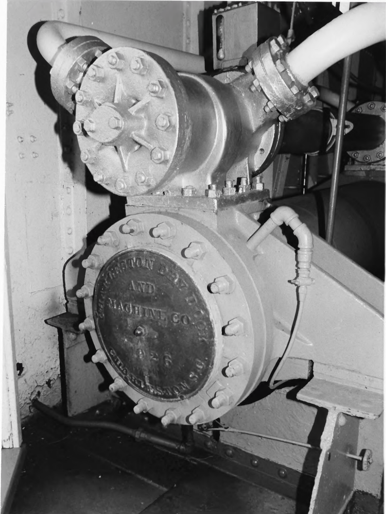
Snagboat Montgomery Pickinsville, Alabama Owner: U.S.Army Corps of Engineers Engine builder's plate on forward cylinder head Photo #5 by Kevin J. Foster, October 26, 1988 Courtesy of: National Park Service
