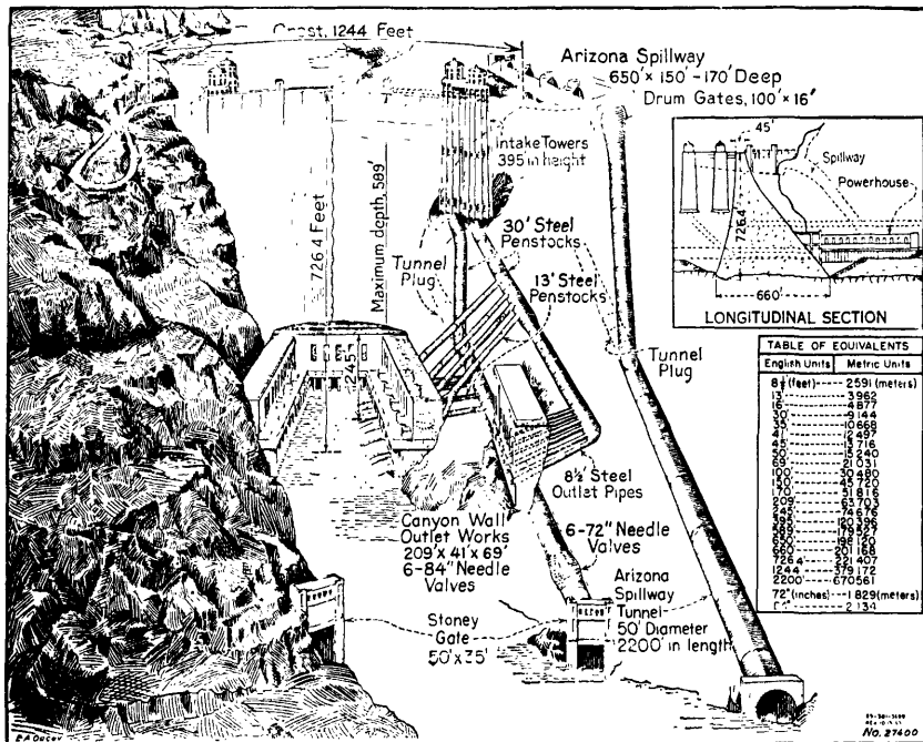
This drawing illustrates the manner in which Hoover Dam works. The Nevada wall of Black Canyon is shown as solid, whereas the Arizona wall is cut away to reveal the intake towers, the spillway, the penstock pipes, and outlet works. Inside the Nevada wall of the canyon a similar set of diversion works has been placed. Principal dimensions are shown.
