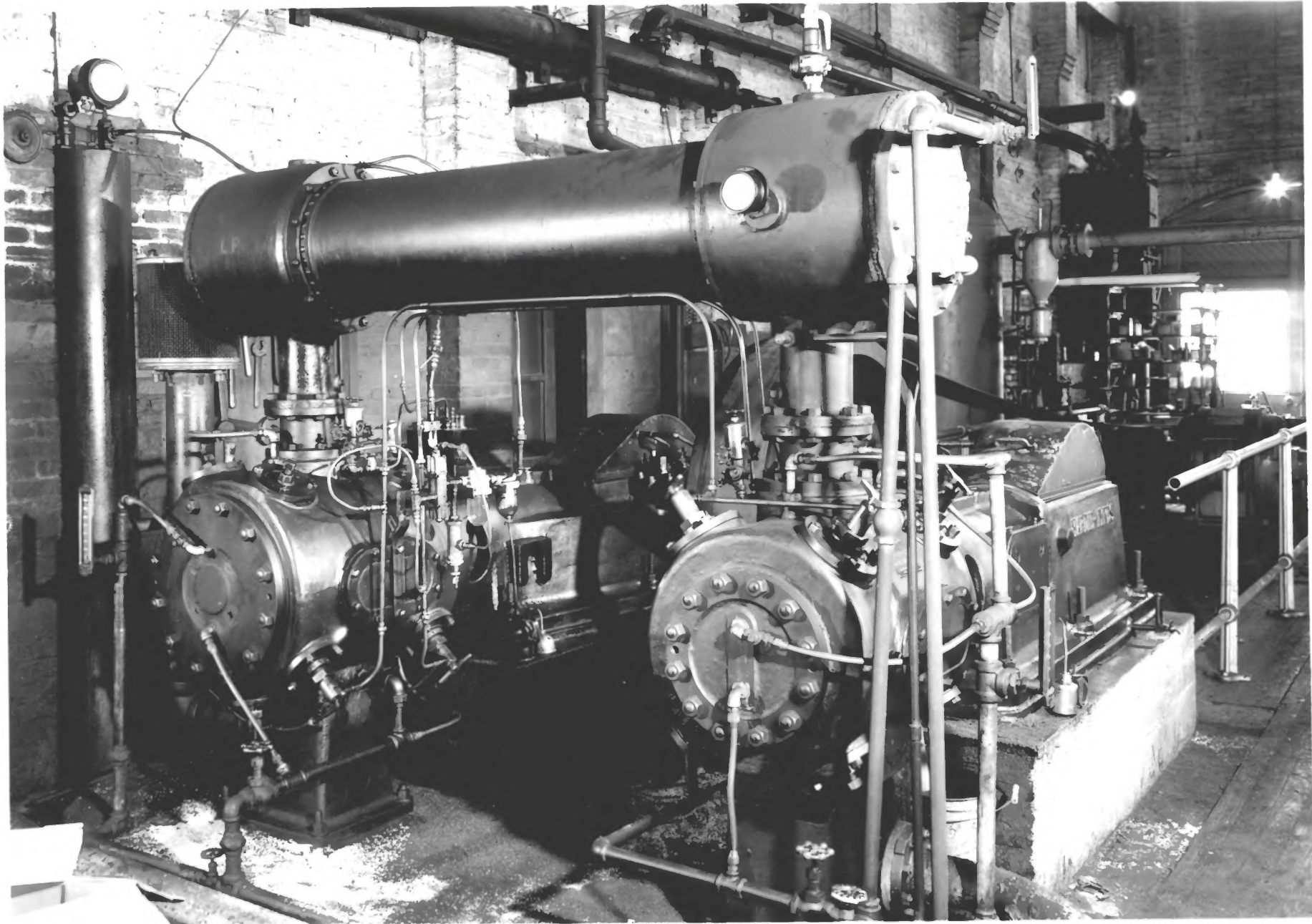
Columbus Iron Works: Power House Air Compressor Engine.
