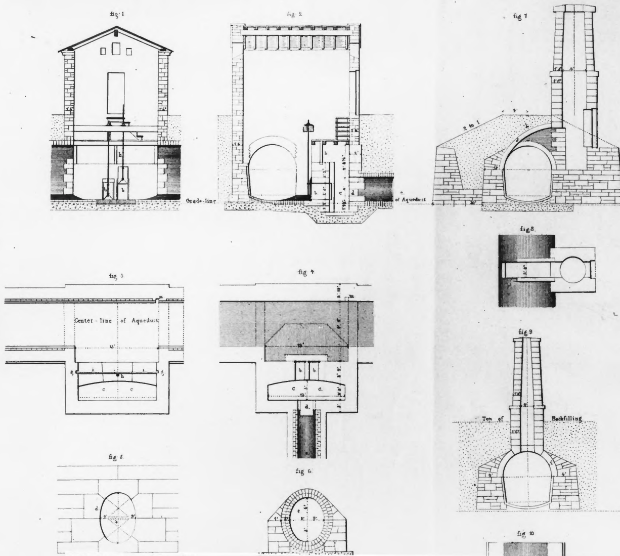
PHOTOGRAPH #7 Croton Aqueduct Westchester, Bronx & New York Counties, New York Sections showing typical construction of the Aqueduct's waste weirs and ventilator shafts. From: Theoph Schramke, Description of the New York Croton Aqueduct, New York, 1843.
