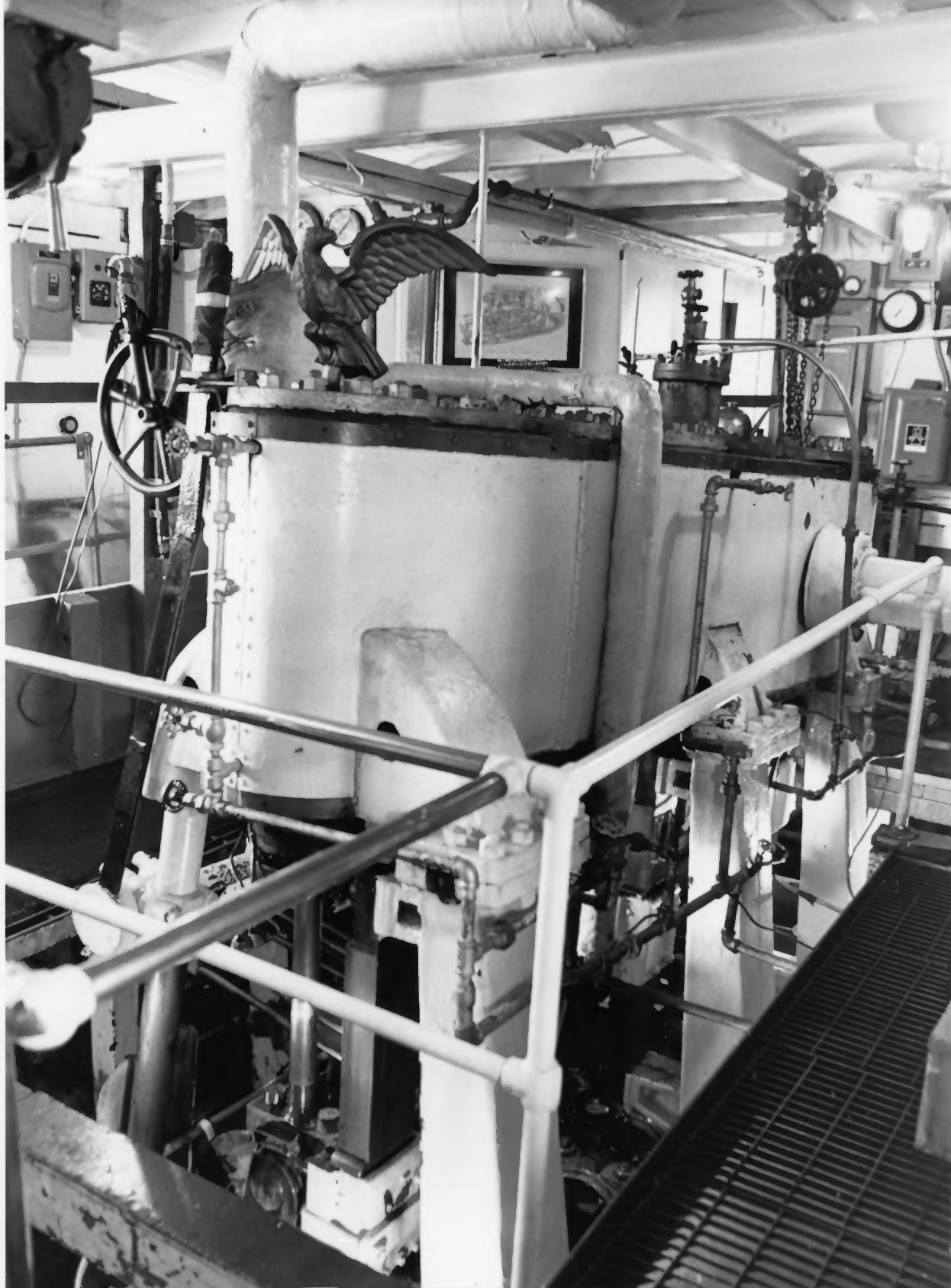
Virginia V , Seattle, Washington Photo courtesy of NPS National Maritime Initiative Photographer: Candace Clifford Original triple expansion marine steam engine, 1991 Photo No. 2
