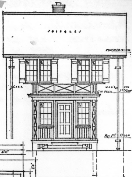
FRONT - ELEVATION
