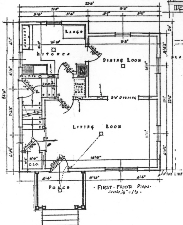
Plan of New Cottages
