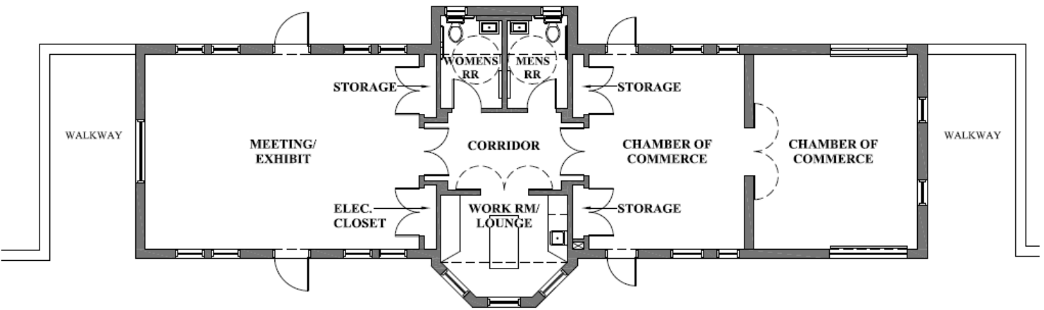
Figure 9: Current floor plan for the Comanche Depot, 2017. Source: Charles W. Ligon AIA Architects, Inc.
