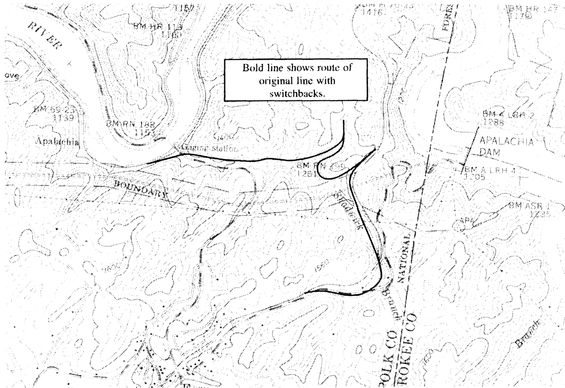
Figure 25: Original Switchback lines of the railroad. (Map courtesy of Louisville & Nashville's Atlanta Division by Michael George.)
