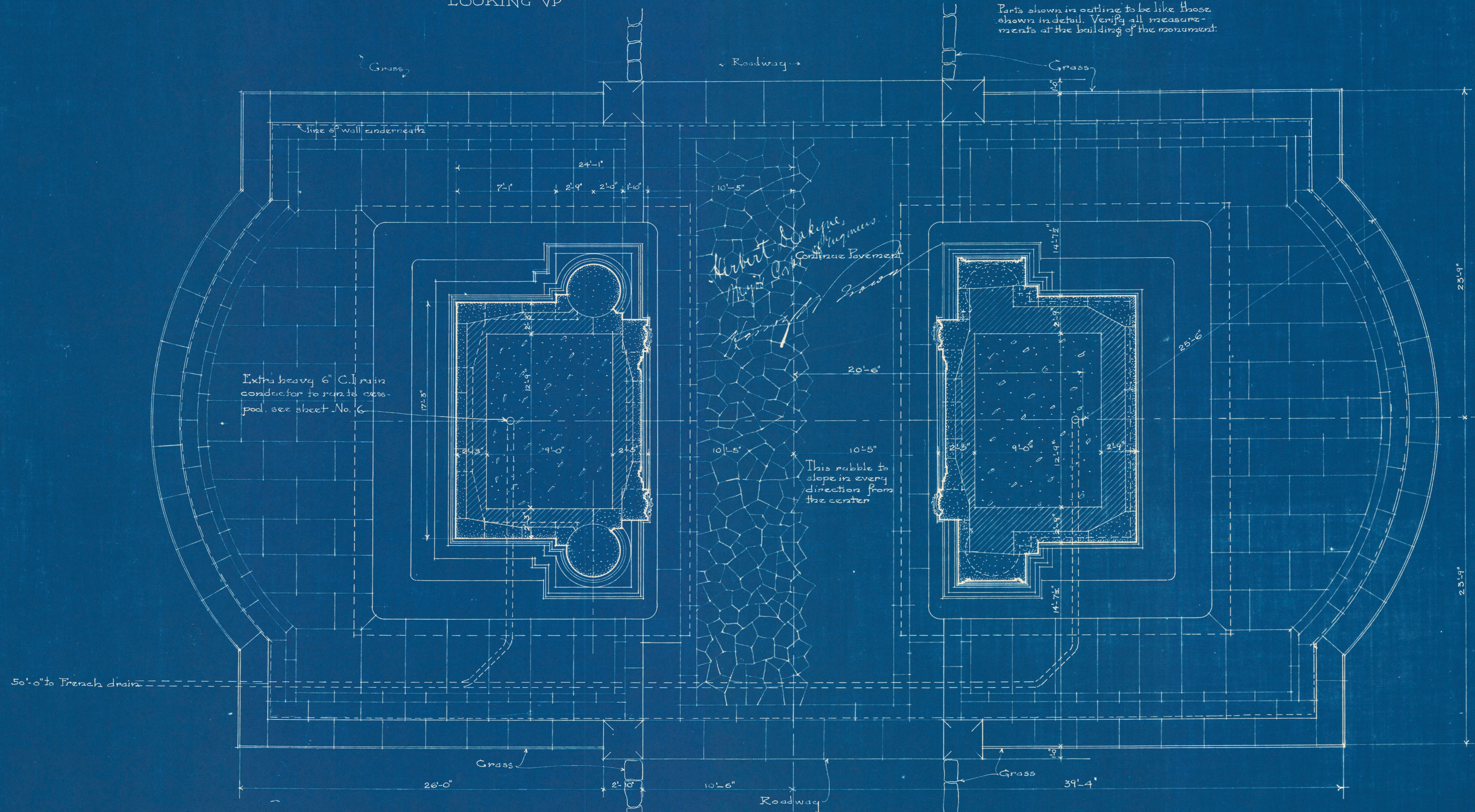
HALF PLAN OF ROOF
