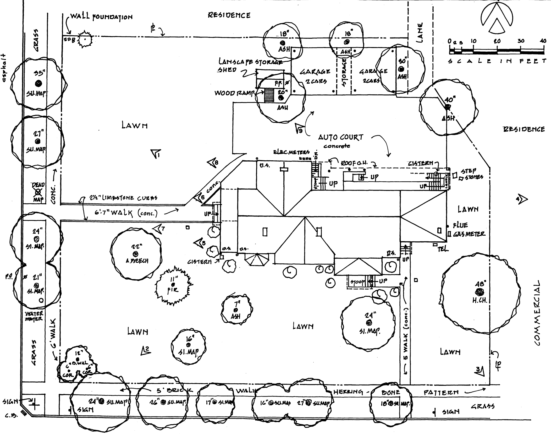
SKETCH PLAN of EXISTING SITE CONDITIONS WELBURN-ROSS HOUSE PRINCETON-GIBSON CO., INDIANA
