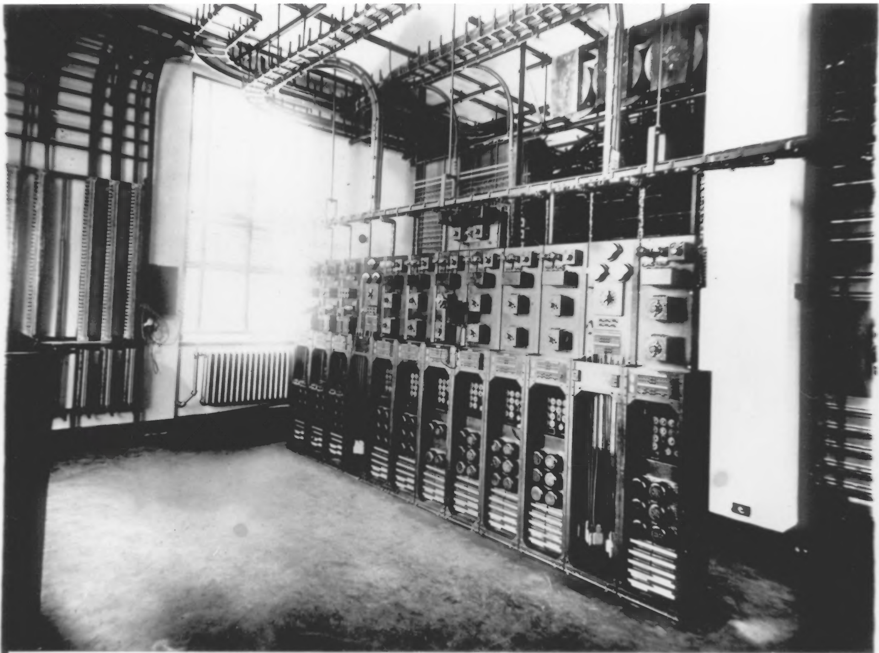
Photo No. 40352 Denmark, S. C. Repeater Office - Line of 2 wire Floor type repeaters
