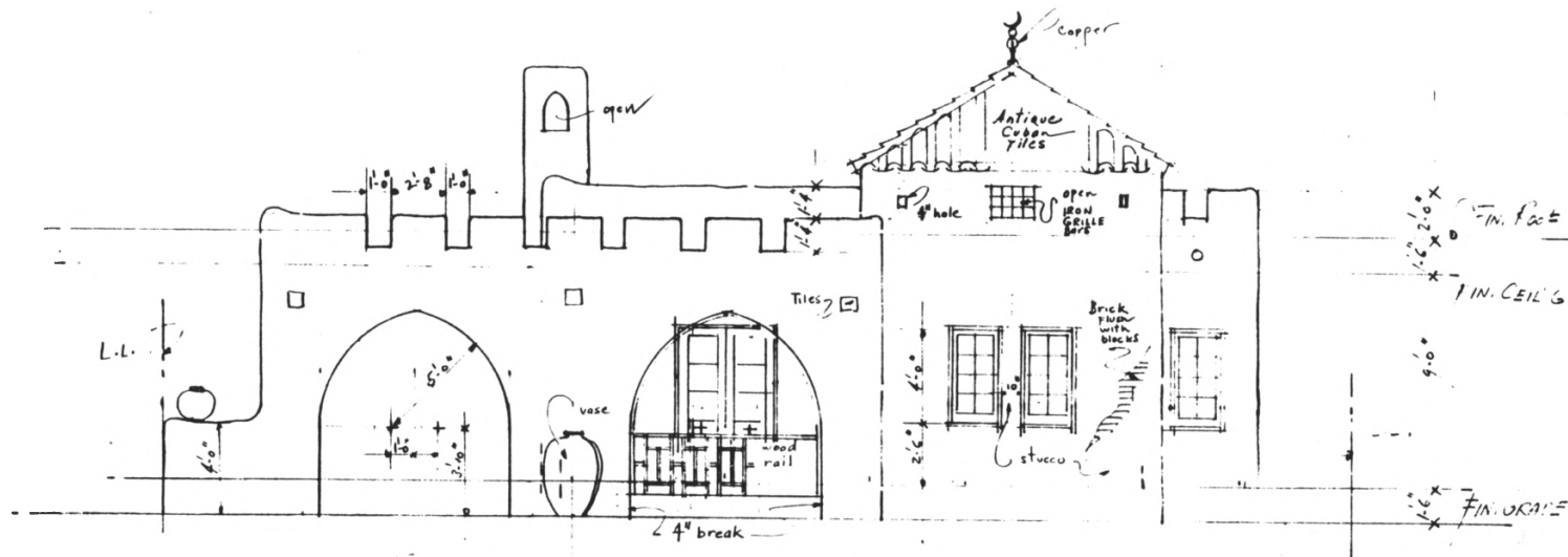
FRONT ELEVATION (SOUTH)
