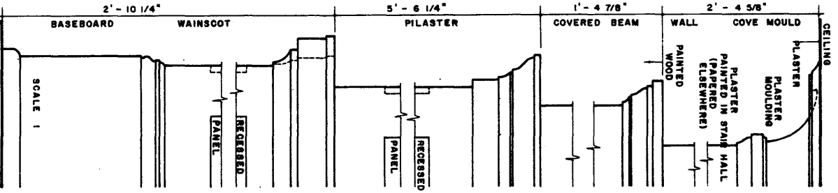
① PILASTER - 1ST FL. ENTRANCE HALL SCALE 1
