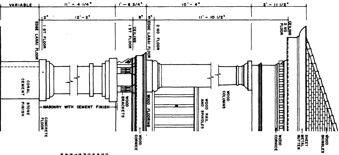
PORTICO - 1ST & 2ND FLOOR LANAIS SCALE 1
