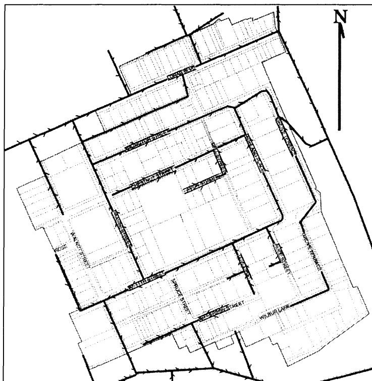
Primary Sanitary Sewer Map (City of Dubuque, 2004)
