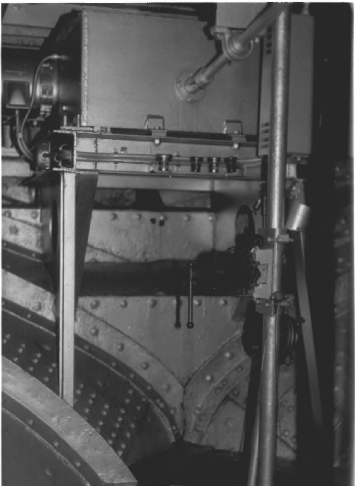
FIREBOAT EDWARD M. COTTER BUFFALO, NEW YORK Owner: BUFFALO FIRE DEPARTMENT STERN SHOWING TYPICAL HULL CONSTRUCTION AND HYDRAULIC STEERING GEAR. Photo #9 by JAMES P. DELGADO, 1989 Courtesy of: NATIONAL PARK SERVICE
