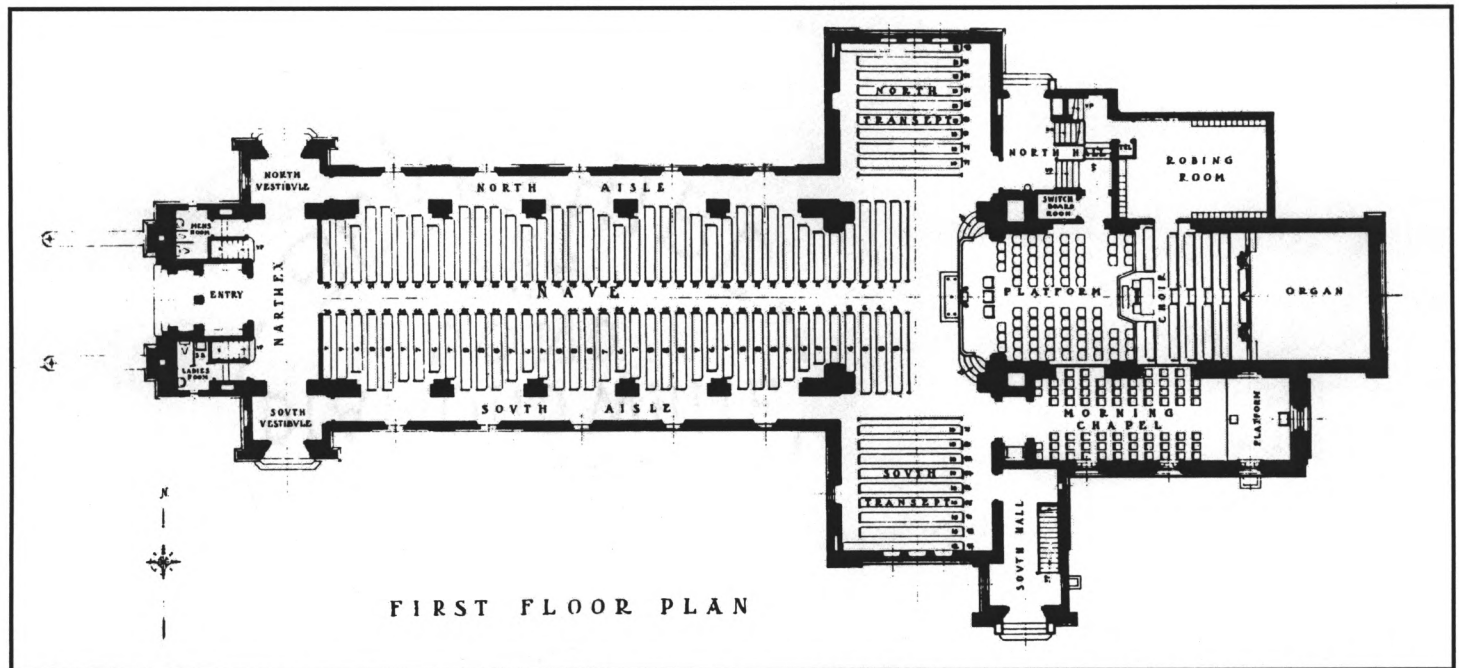
Figure 1. Architect John Gray's plans for Shove Memorial Chapel are on display in the Chapel Office. This plan for the first floor identifies the principal areas of the building's interior. SOURCE: Fuller, ed., This Glorious and Transcendent Place , 6.
