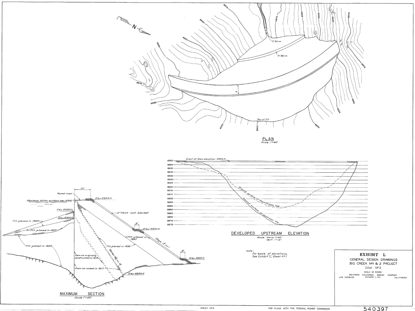
Figure 7: Huntington Lake Dam No. 3 General Design Drawings, 1954. Drawing No. 540397. On file at SCE Northern Hydro Headquarters.
