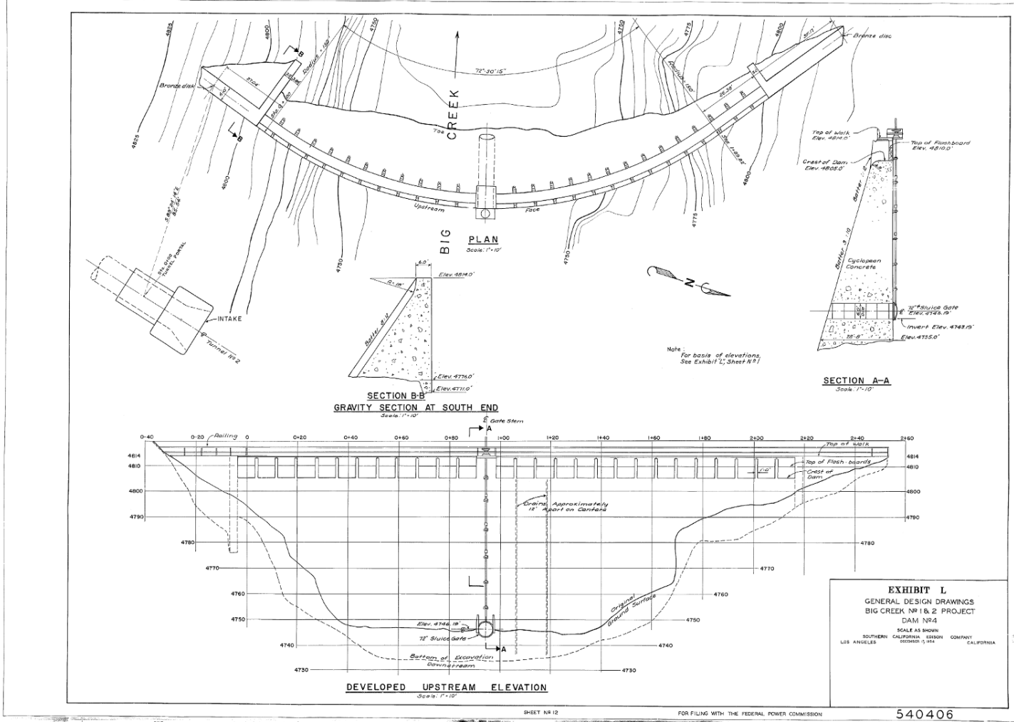
Figure 18: Dam No. 4 General Design Drawing, 1954. On file at SCE Northern Hydro Headquarters.
