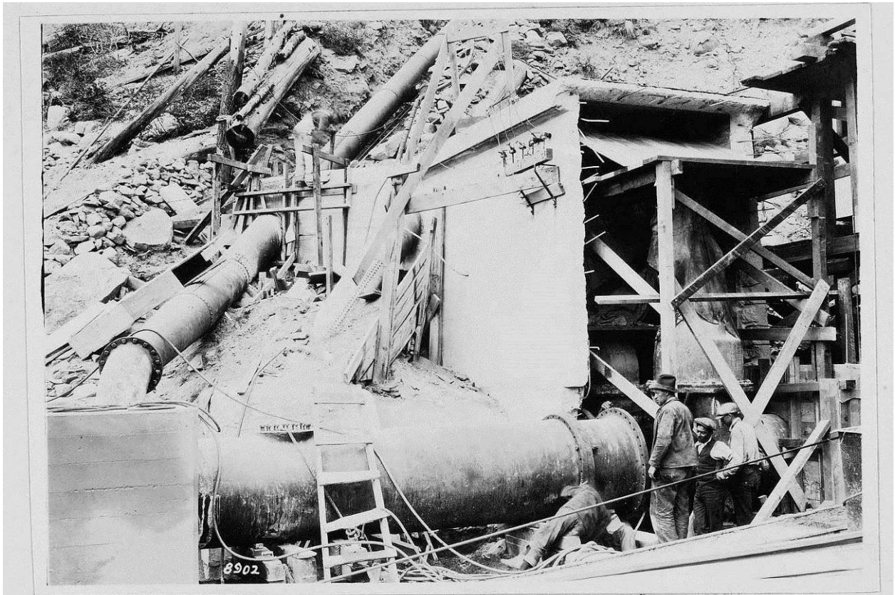
Figure 10: Tunnel No. 1 Flowline showing the penstocks, gate and vent pipes for Powerhouse No. 1, 1923. Image No. SCE-02-08902, Huntington Digital Library.
