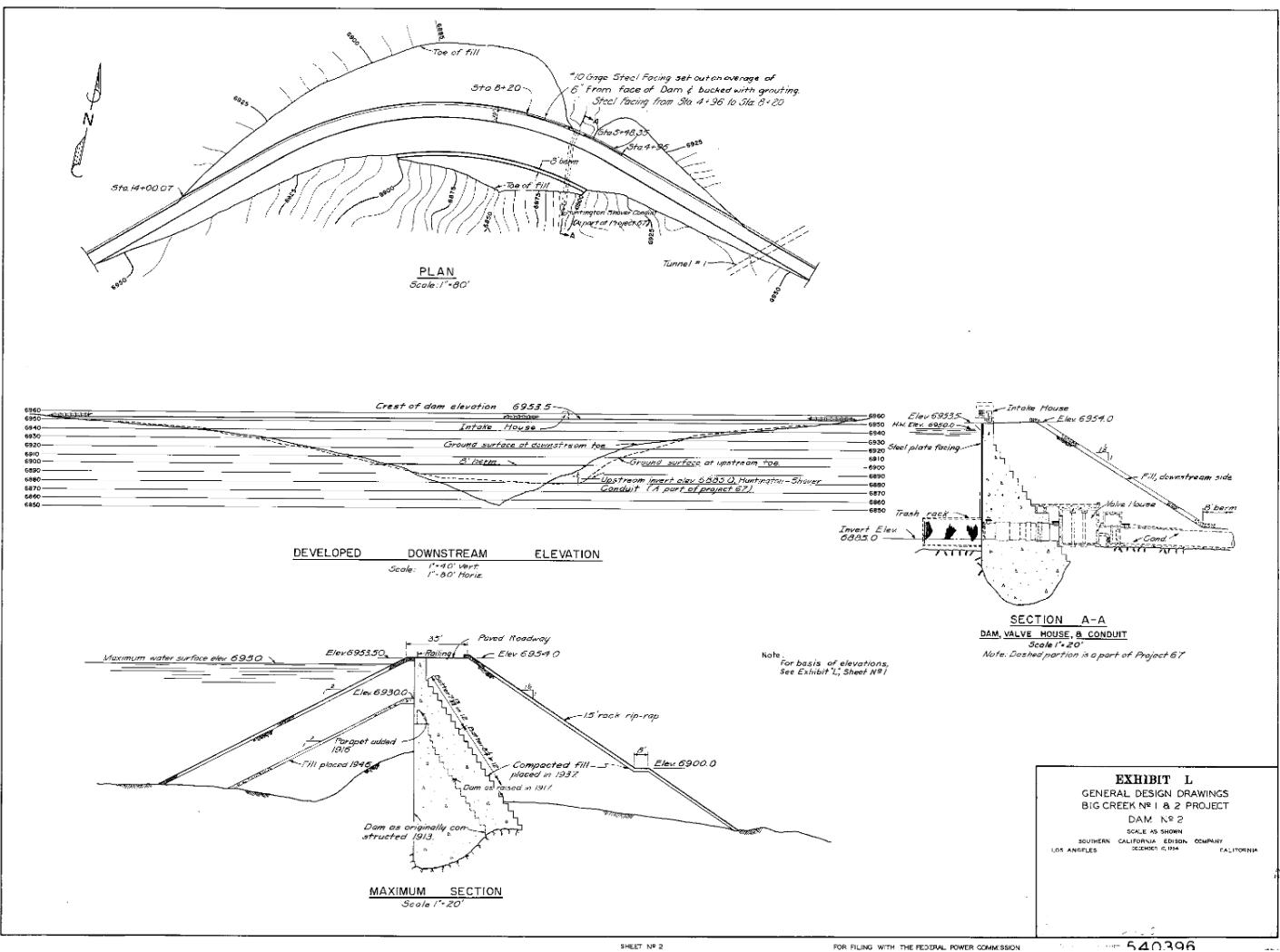
Figure 5: Huntington Lake Dam No. 2 General Design Drawings, 1954. On file at SCE Northern Hydro Headquarters.
