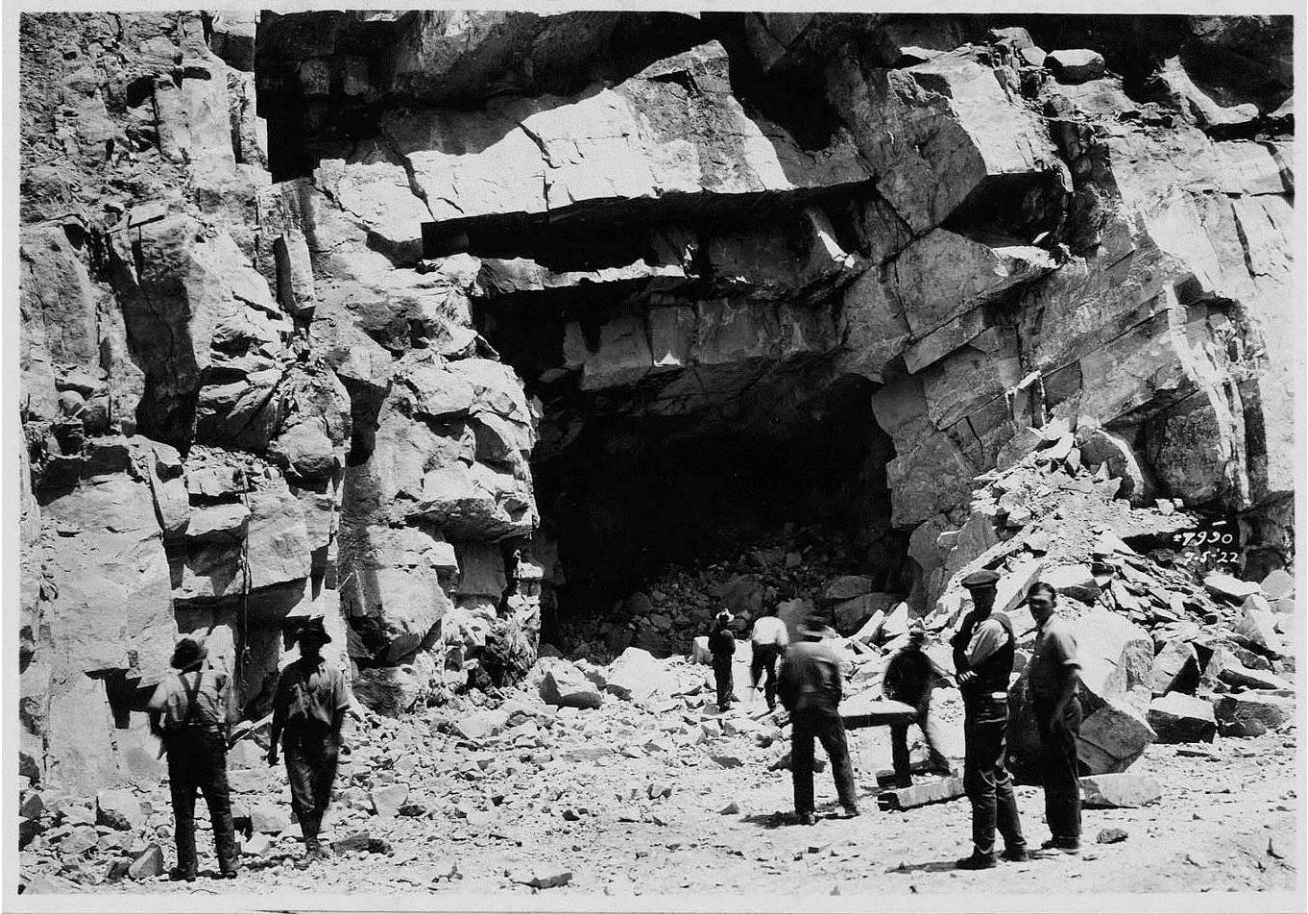
Figure 42: Tunnel No. 3-Adit No. 35, 1922. Image No. SCE-02-07990, Huntington Digital Library.
