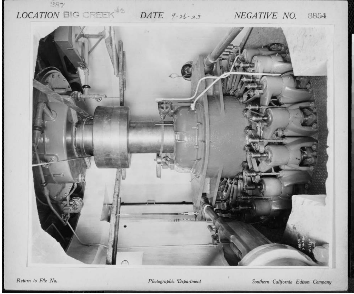
Figure 52: Powerhouse No. 3 close-up of turbine, 1923. Image No. SCE-02-08854, Huntington Digital Library.
