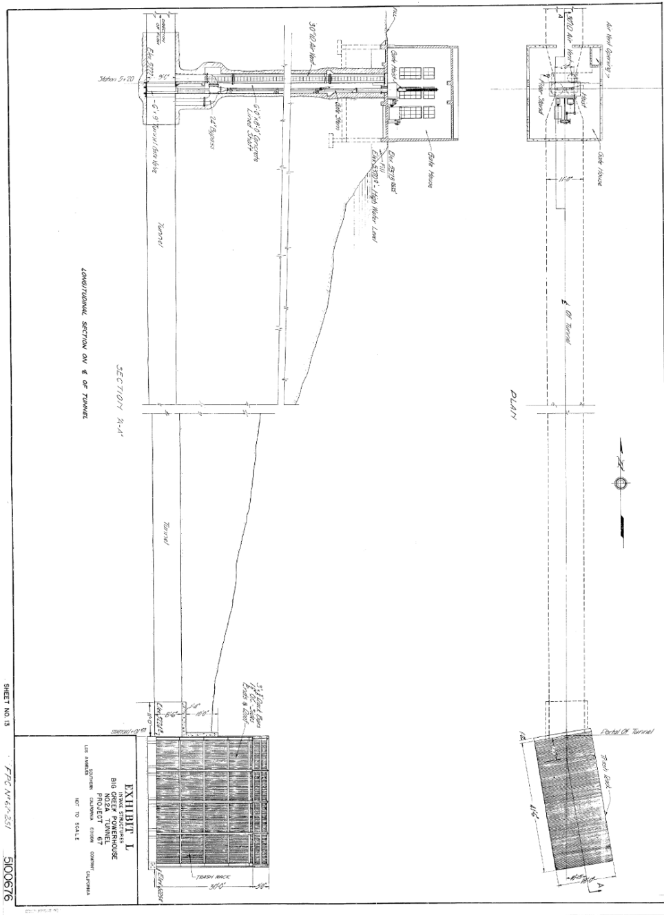
Figure 29: Tunnel No. 5 Intake General Design Drawing, n.d. Drawing No. 5100676, on file at SCE Northern Hydro Headquarters.
