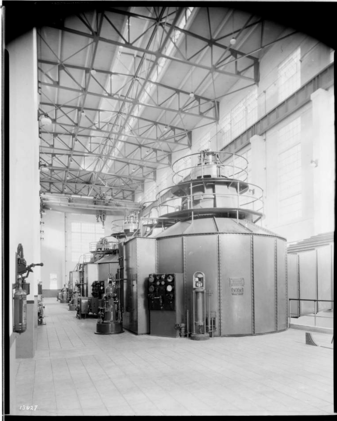
Figure 53: Powerhouse No. 3 Generator Room Floor, 1926. Image No. SCE-02-13827, Huntington Digital Library.
