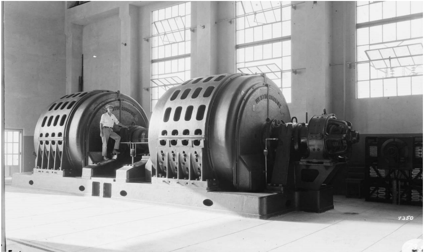
Figure 102: Vestal Substation Interior, synchronous condensers, 1921. Image No. SCE-02-07350, Huntington Digital Library.
