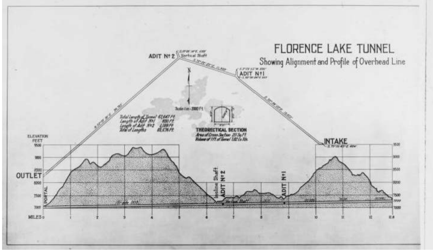
Figure 61: Profile Drawing of Florence/Ward Tunnel, 1925. Image No. SCE-02-13030, Huntington Digital Library.
