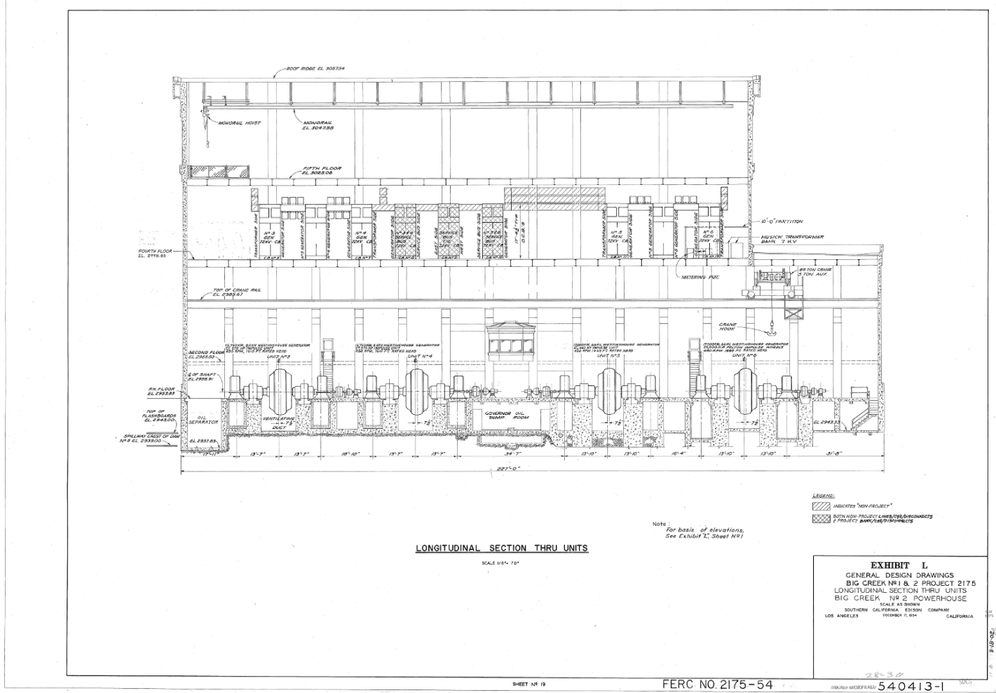
Figure 26: Powerhouse No. 2 General Design Drawing, 1954. Drawing No. 540413-1. On file at SCE Northern Hydro Headquarters.
