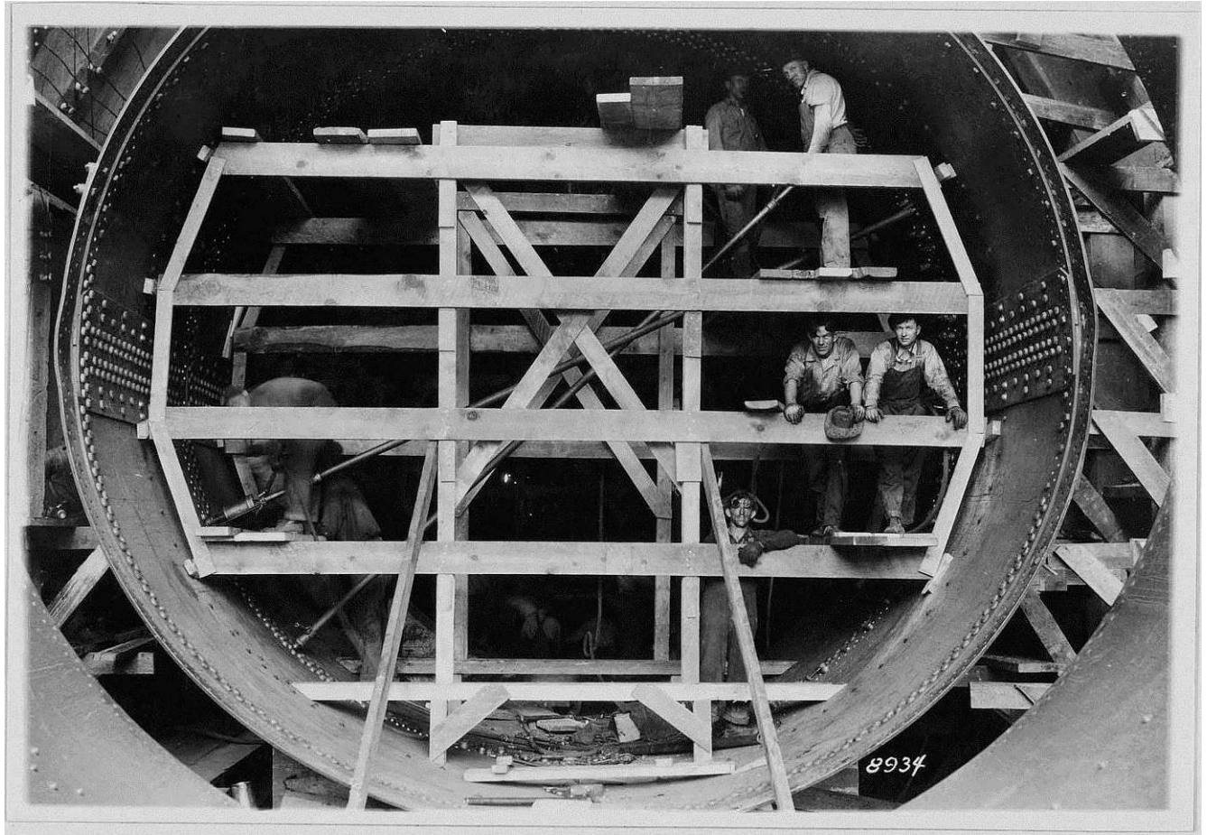
Figure 44: Section of Riveted Steel Pipe in Tunnel No. 3, 1923. Image No. SCE-02-08934, Huntington Digital Library.
