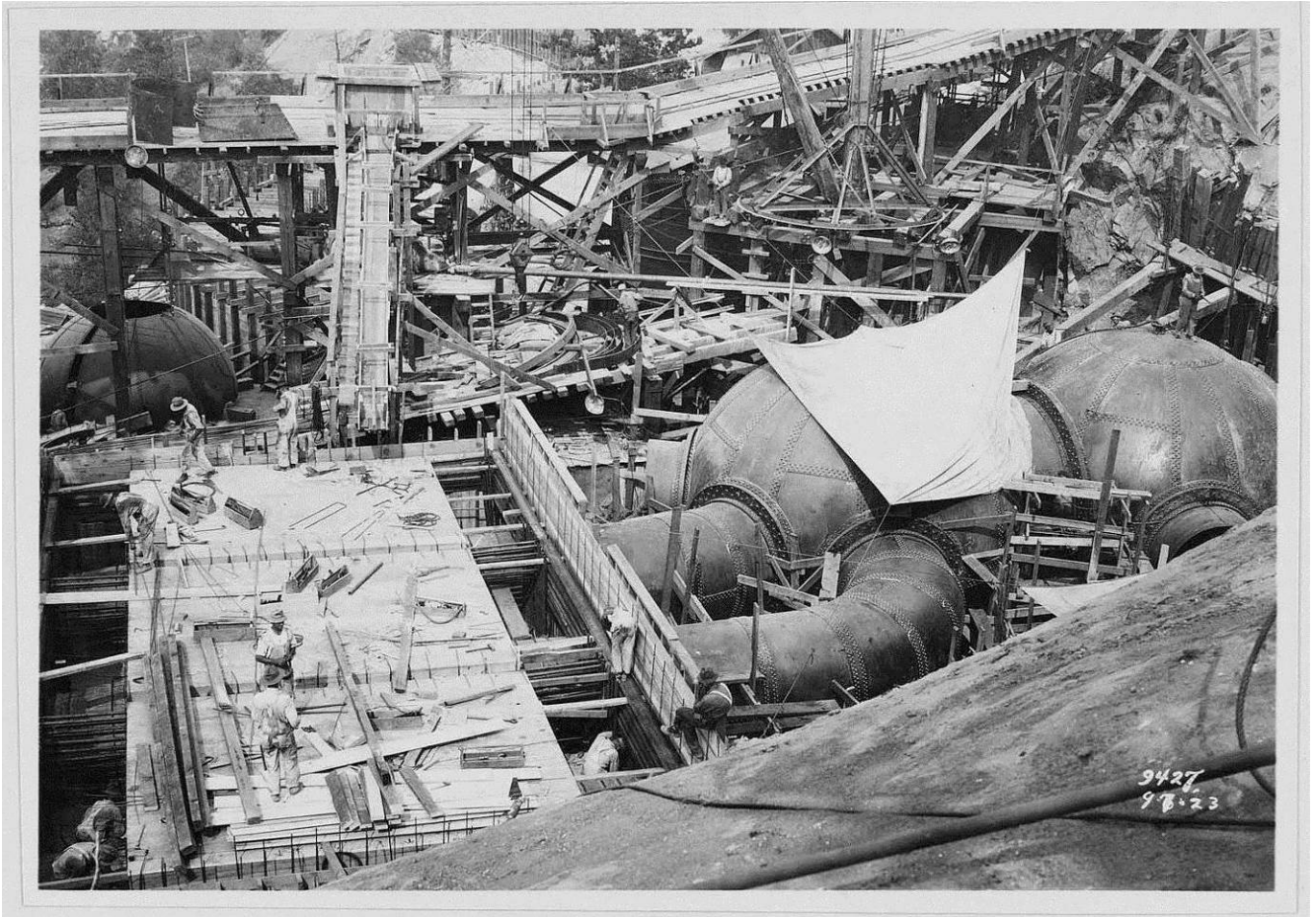
Figure 50: Powerhouse No. 3 Penstock Manifold under construction, 1923. Image No. SCE-02-09427, Huntington Digital Library.
