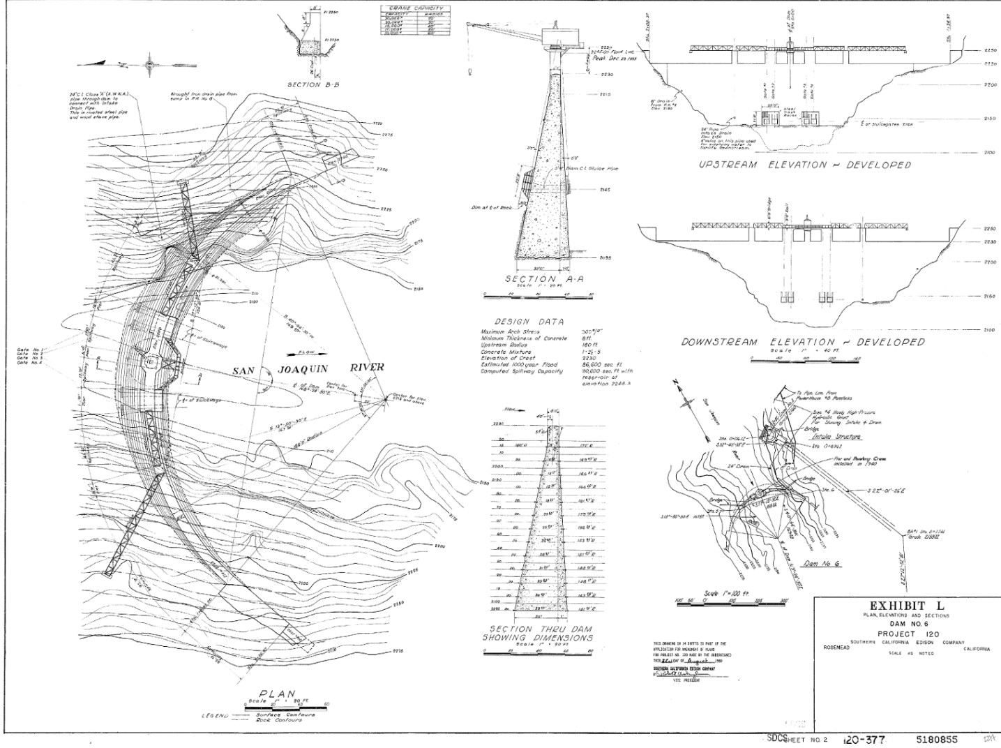
Figure 48: Dam No. 6 General Design Drawings, n.d. Drawing No. 5100666-1, SCE Northern Hydro Headquarters.
