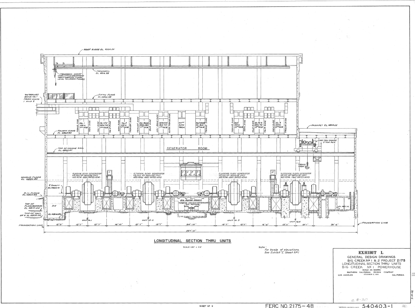
Figure 16: Powerhouse No. 1 Design Drawing, 1954. On file at SCE Northern Hydro Headquarters.
