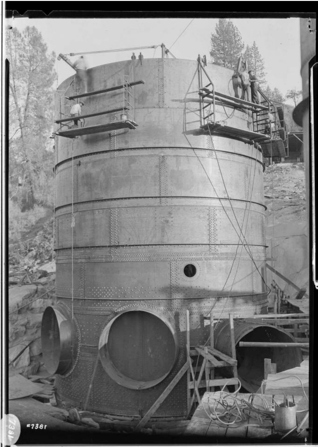
Figure 33: Powerhouse No. 8 Surge Tank, 1921. Image No. SCE-02-07381, Huntington Digital Library.
