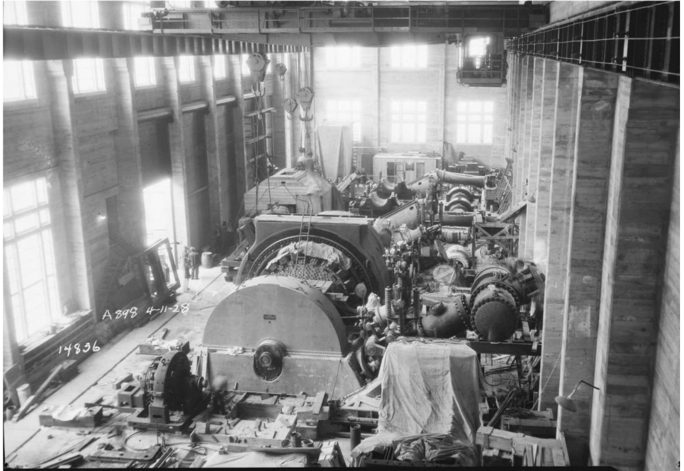
Figure 87: Powerhouse No. 2A Generator Floor, 1928. Image No. SCE-02-14836, Huntington Digital Library.
