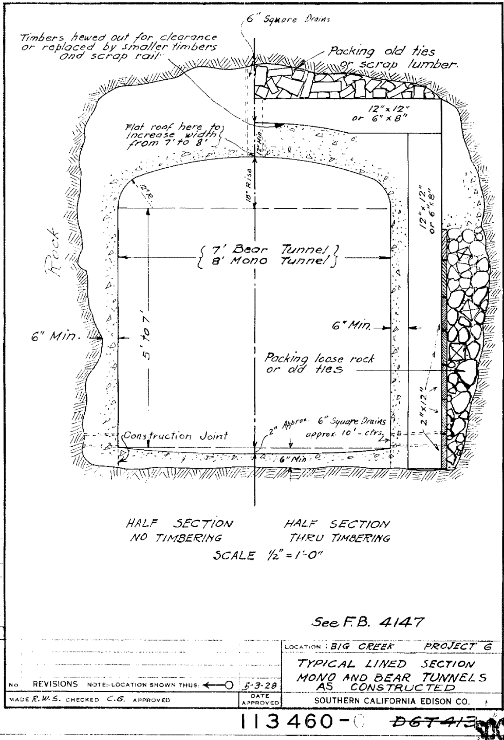
Figure 78: Typical Lined Sections Mono and Bear Tunnels, 1929. Drawing No. 113460, SCE Northern Hydro Headquarters.
