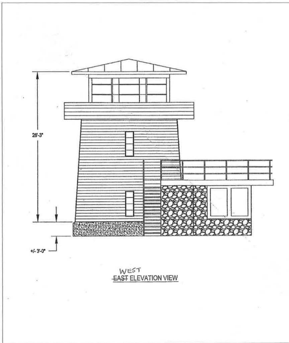
Figure 9. Clay Butte Lookout, West Elevation View (Source: United States Department of Agriculture Forest Service Region 2, Shoshone National Forest: Construction Drawings for Clay Butte Lookout Tower Repairs, 2010)
