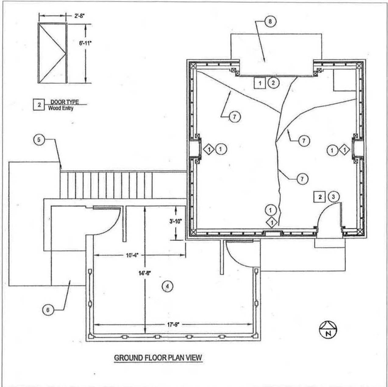
Figure 5. Clay Butte Lookout, Ground Floor Plan View (north arrow added; numbers are keyed to renovation details) (source: United States Department of Agriculture Forest Service Region 2, Shoshone National Forest: Construction Drawings for Clay Butte Lookout Tower Repairs, 2010)
