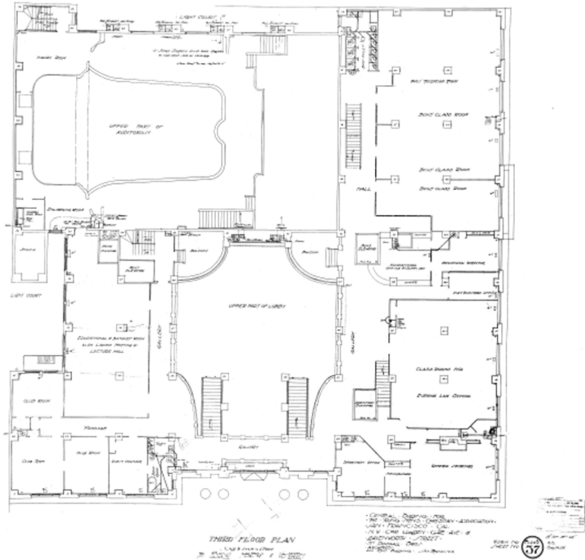
Figure 4. 1908 Drawings – Third Floor
