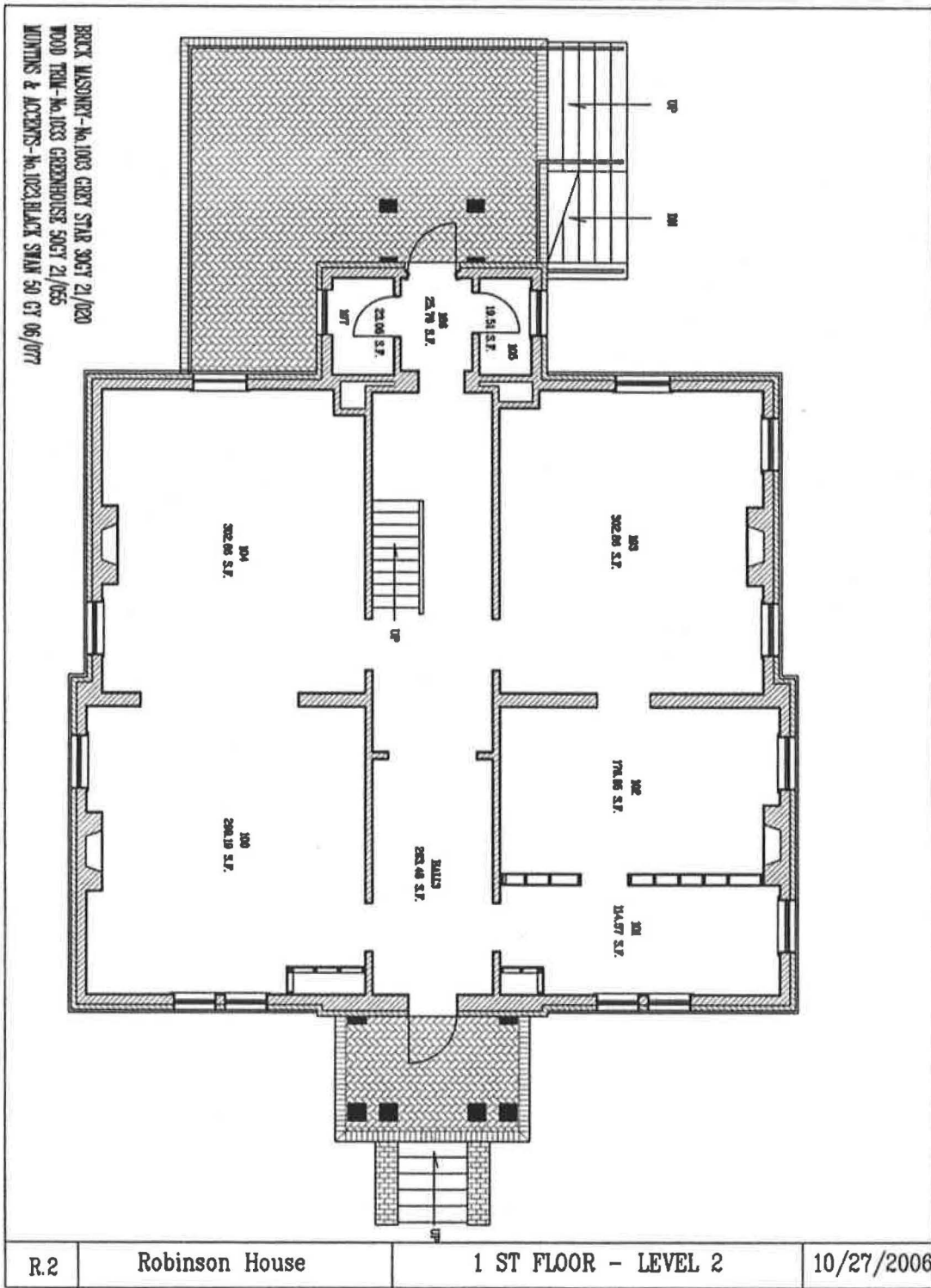
Fig. 2. Floor plan, first floor. Margaret R. and Robert M. Freeman Library VMFA.
