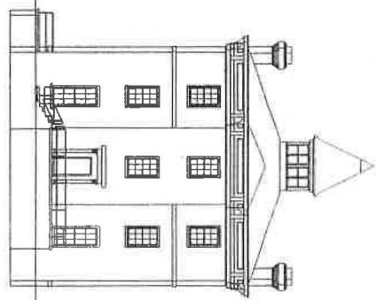
NORTH ELEVATION
