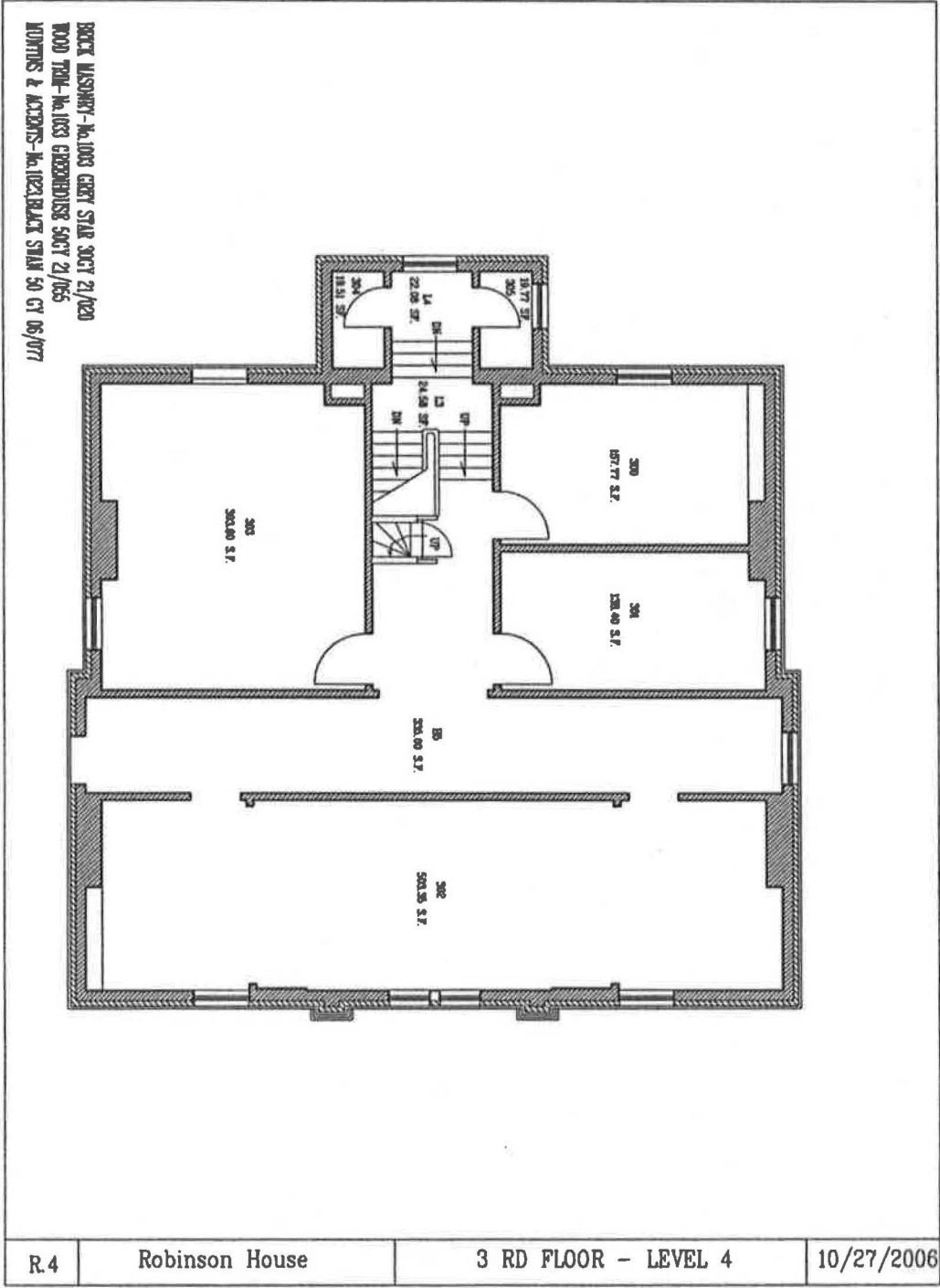
Fig. 4. Floor plan, third floor. Margaret R. and Robert M. Freeman Library VMFA.
