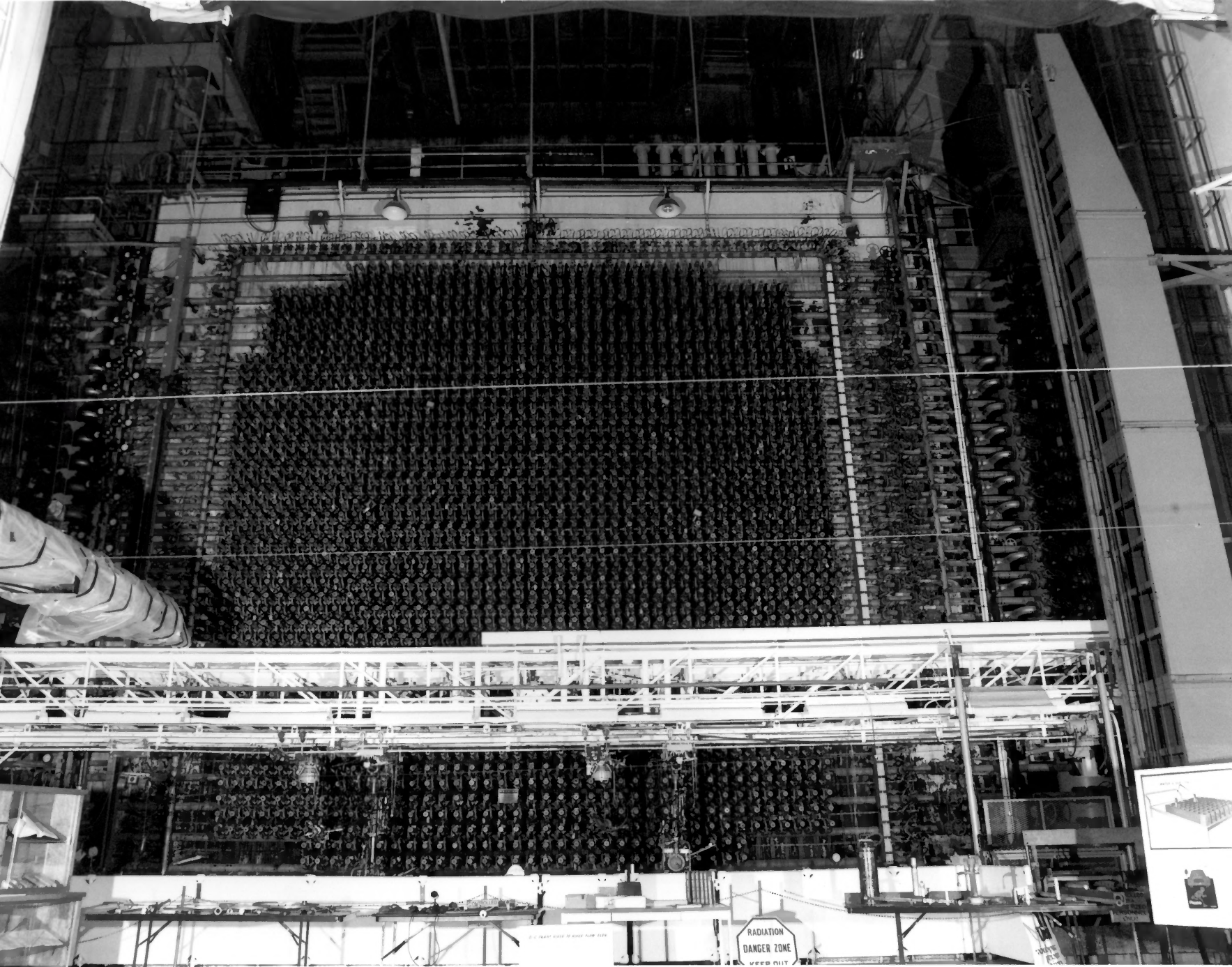
Figure 6. The front (loading) view of the 100-B Reactor as it appears today.
