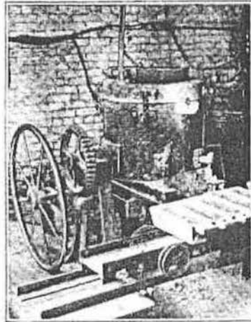
A FIRST COMMERCIAL AJAX-WYATT FURNACE
