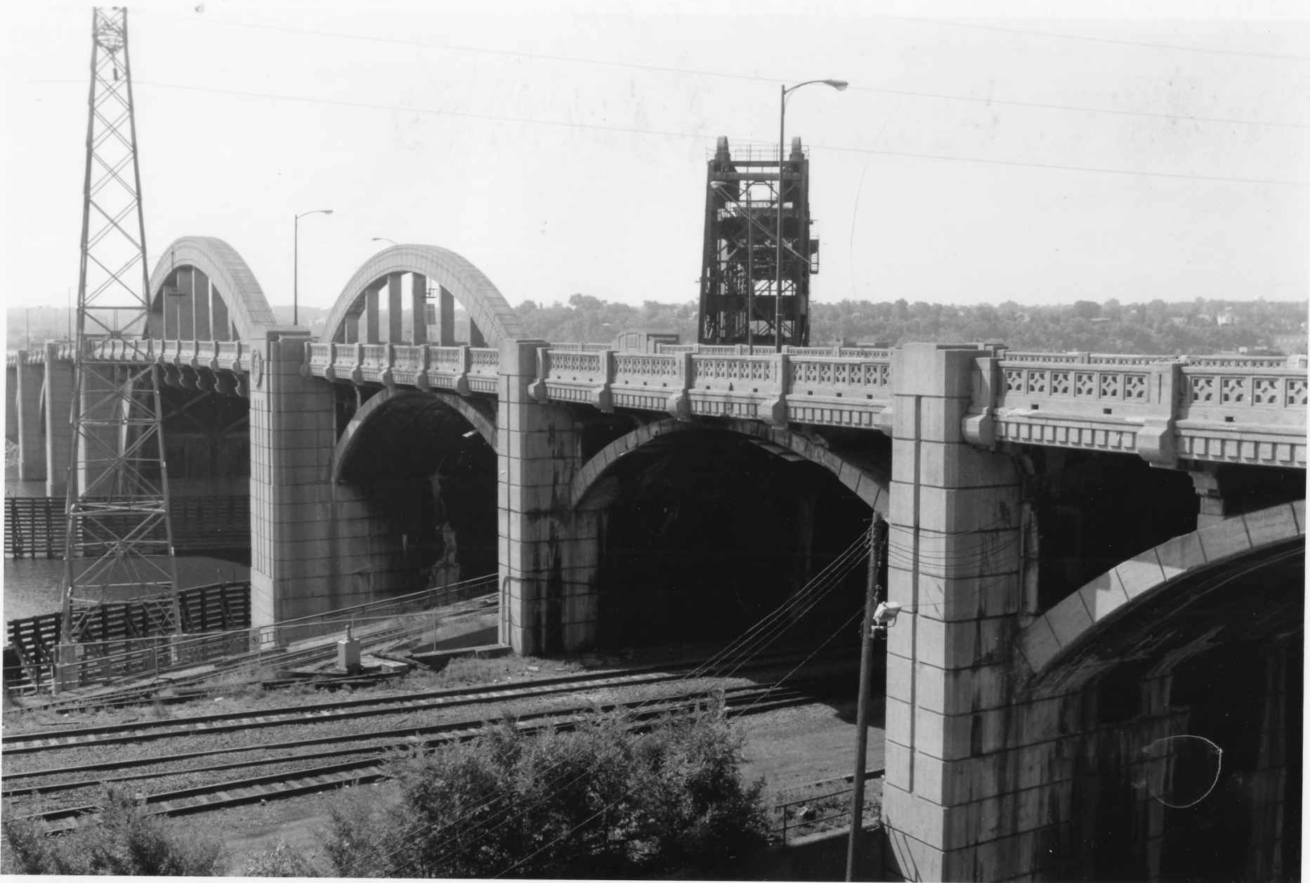
ROBERT STREET BRIDGE, NO. 9036 RAMSEY CO., MN PHOTO I.D. 09969 #8
