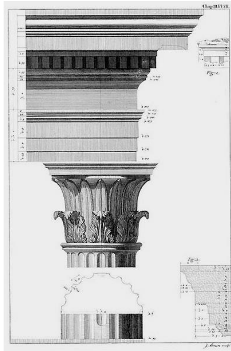
Image L Detail of Capital on Entrance Portico and Corinthian Capital from James Stuart and Nicholas Revett, Tower of the Winds, The Antiquities of Athens , Vol. I, Chapter 3, Plate 7, London: John Haberkorn, 1762.
