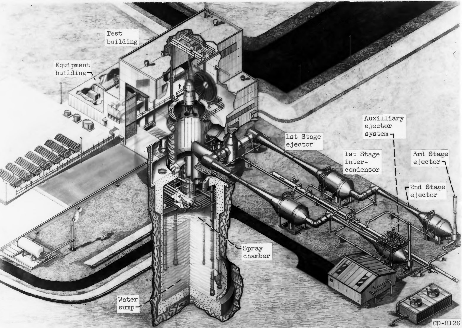
Figure 4. - Cutaway view of Spacecraft Propulsion Research Facility.
