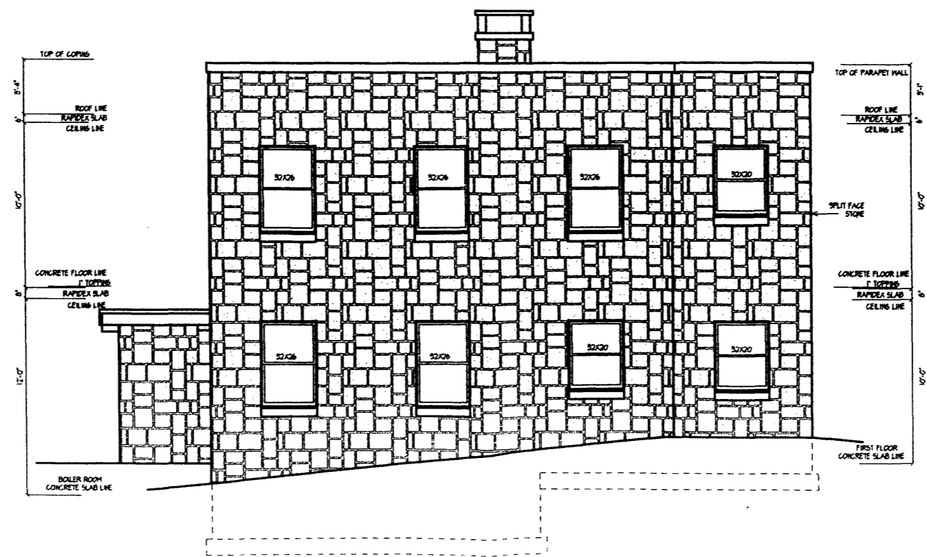
BACK ELEVATION
