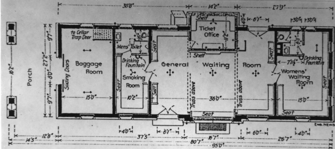
Fig. 6. PLAN OF STATION AT RICHMOND, IND.
