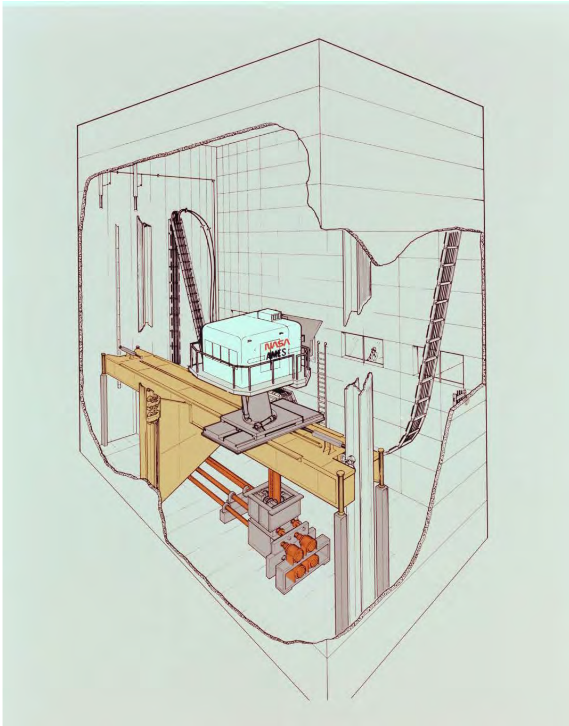
Figure 4. Cutaway illustration of the Vertical Motion Simulator (VMS)
