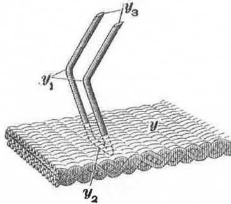
Figure 1 Phantom view of fabric-based card clothing Showing foundation (y) and inserted wire staple (y 1 -y 3 ) International Library of Technology, Vol. 76
