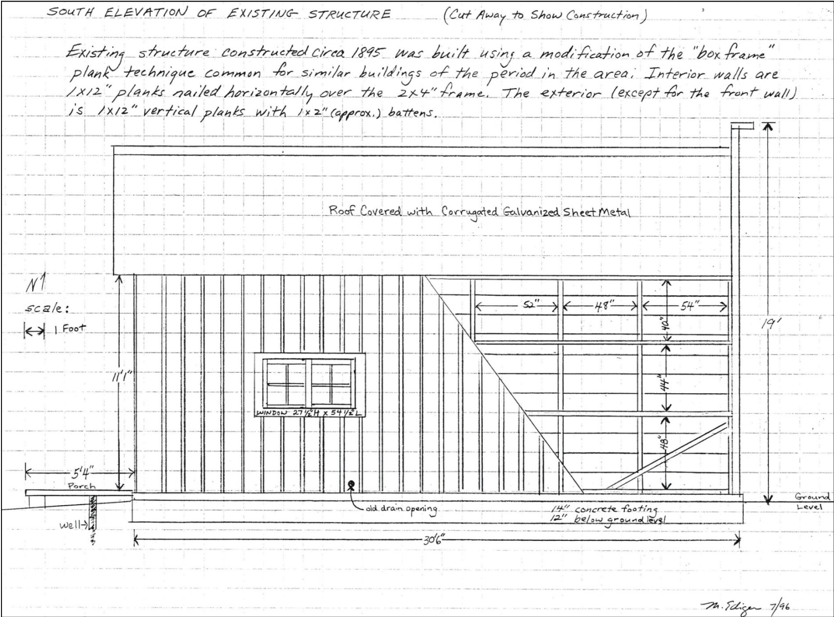
Figure 5. Wall construction detail, showing widely spaced framing members, vertical exterior boards, and horizontal interior boards. Courtesy Michael Ediger, July 1996.
