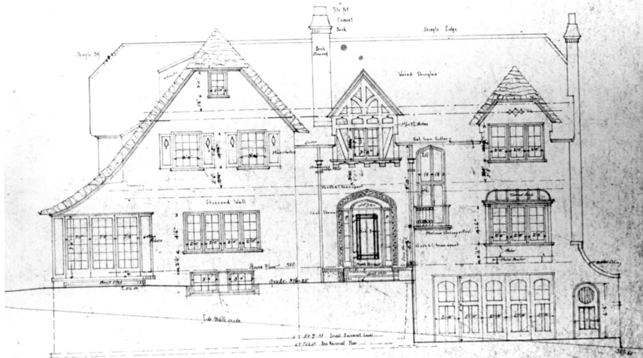
FRONT ELEVATION
