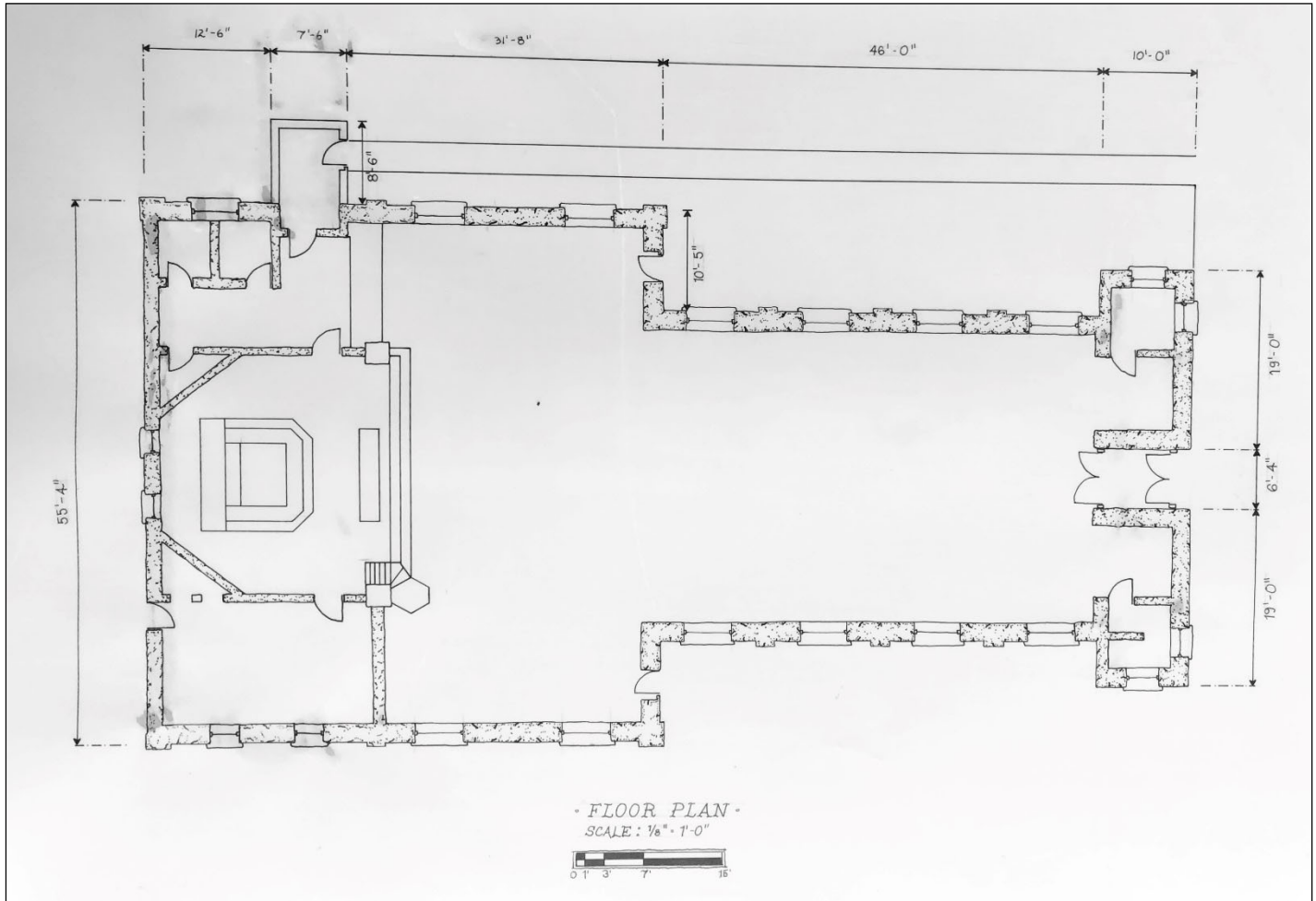
Figure 13. Phillips B. Gallegos prepared this measured drawing of the floorplan of Our Lady of Guadalupe in 1989 as part of a study of Hispanic religious architecture in the San Luis Valley. North is to the top of the page. Courtesy of Phillip B. Gallegos, Our Lady of Guadalupe, Conejos, Colorado, Measured drawing, August 1989, Phillip B. Gallegos Hispanic Religious Architecture of San Luis Valley, Center for Southwest Research, University of New Mexico, Albuquerque, New Mexico.
