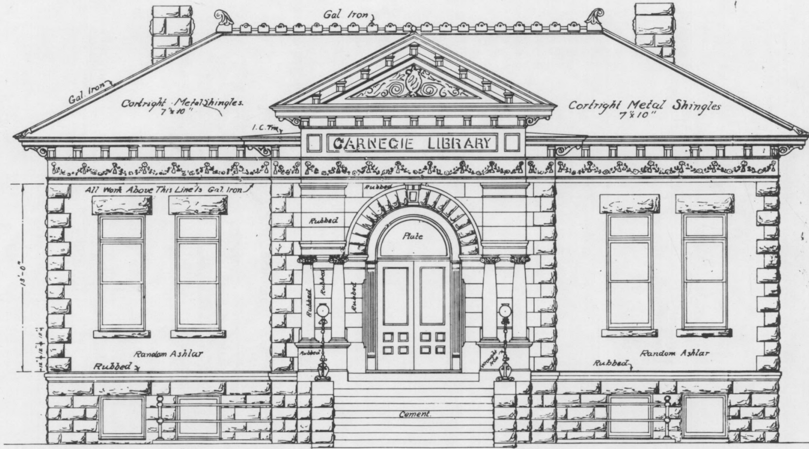
— FRONT ELEVATION —
