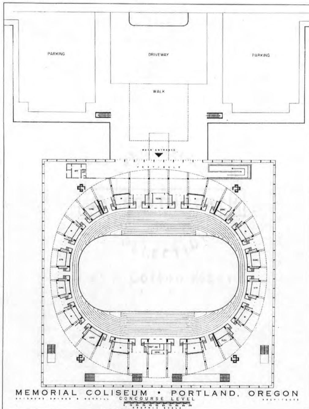
Figure 2. Memorial Coliseum Entry-Level Floor Plan. Drawing by SOM, approximately 1959
