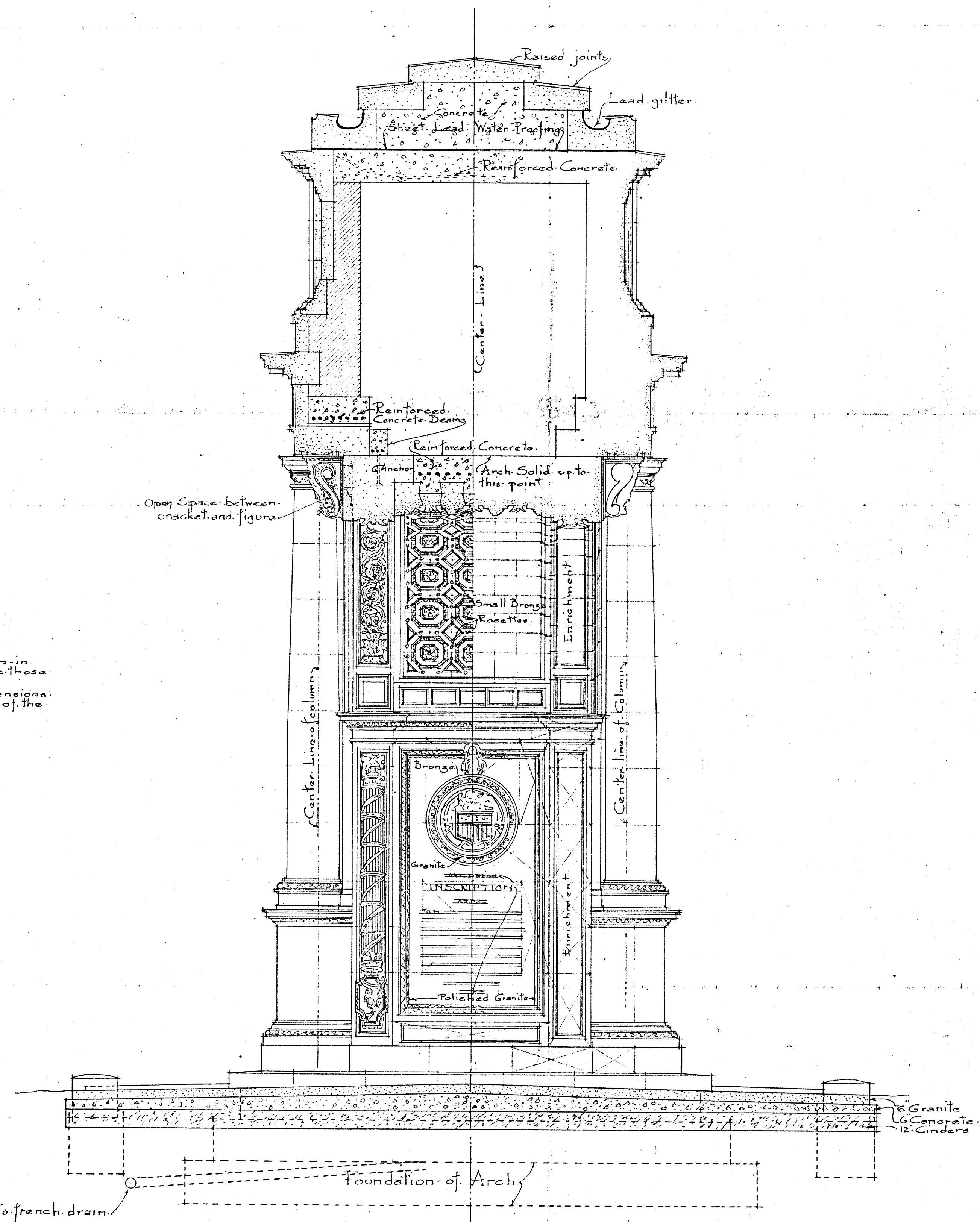
SECTION
