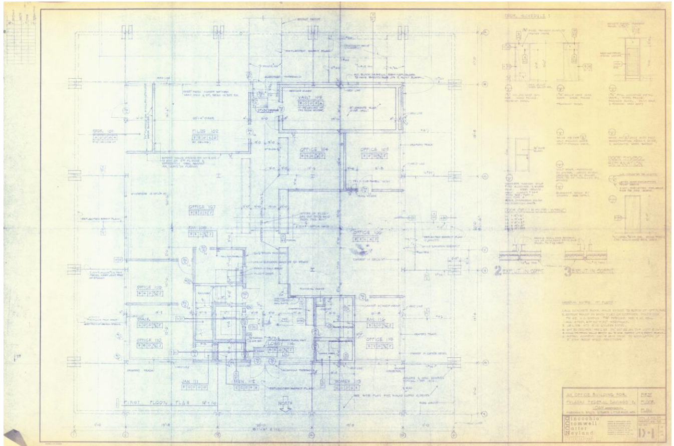
Figure 5: First floor plan of the Block Realty Building, 1964.
