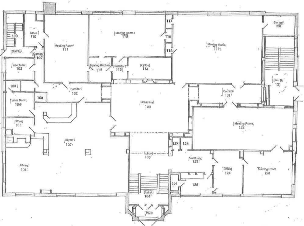
EXISTING MAIN (FIRST) LEVEL PLAN
