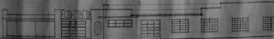
SIXTH ST. ELEVATION SCALE 1/8" = 1'-0"
