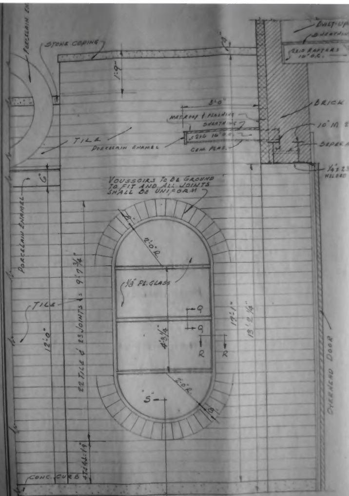
DETAIL ELEVATION OF DISPLAY WINDOW SCALE 1/2" = 1'-0"
