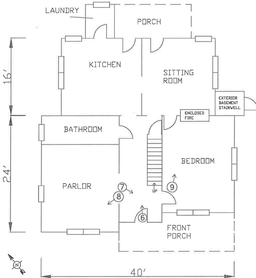
Figure 5: First Floor Plan and Photographic Locations (Not to Scale)
