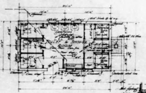
FLOOR PLAN Scale 1/4" = 1'-0"
