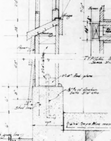
TYPICAL WALL & WINDOW SECTION Scale 3/16" = 1'-0"
