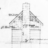
RIGHT SIDE Scale 1/4" = 1'-0"
