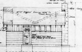
FRONT ELEVATION Scale 1/4" = 1'-0"
