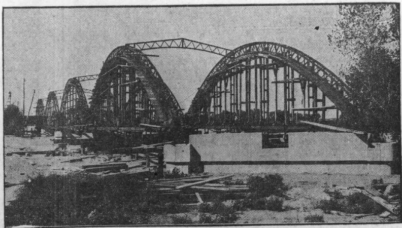
South Lawrence Avenue Bridge of Marsh Arch Design Now Under Construction on Highway 81.
