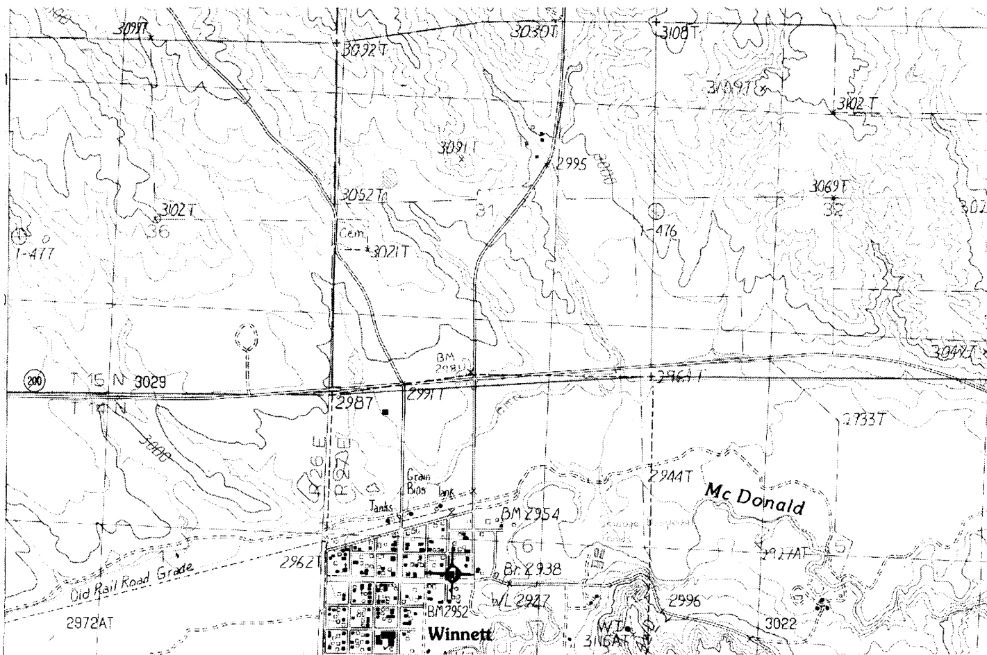
Location of the Winnett Block Winnett North, MT, Provisional Edition, 1986, 7.5' quadrangle
