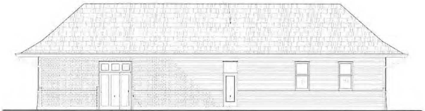
10 WEST ELEVATION - NEW 1/4" = 1'-0"
