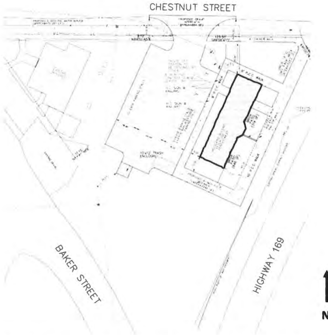
Figure 8: New Location Site Plan showing the boundaries of the nominated property which is the building itself. It measures 73' x 21'. The depot is set back approximately 50' feet from Highway 169. Courtesy of Simonson & Associates Architects, January 2014.
