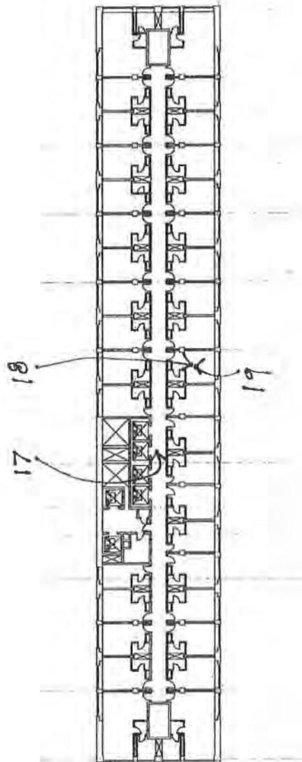
Figure 16. Existing typical hotel floor plan, floors 9 through 18, courtesy of owner, and photo key
